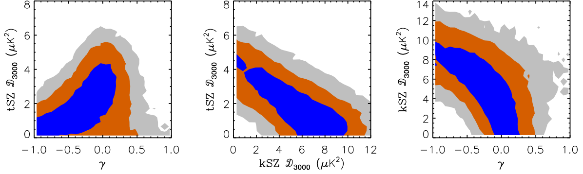
FIG. 12.— 2D likelihood contours for tSZ-DSFG correlation chains in which kSZ is allowed to vary. The 68%, 95% and 99.7% likelihood contours are marked with blue, orange and gray respectively. From left to right: tSZ power vs. correlation coefficient \gamma ; tSZ power vs. kSZ power, marginalized over \gamma (and foreground terms); and kSZ power vs. \gamma .
