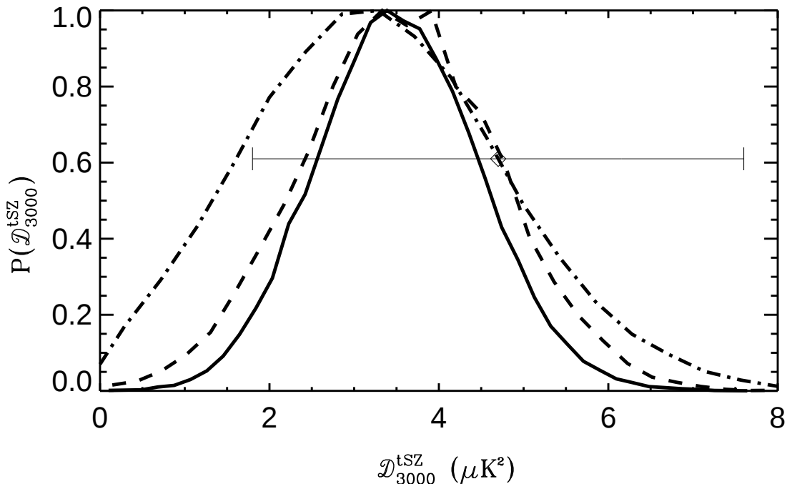
FIG. 6.— The solid black line shows the 1D likelihood surface for D_{3000}^{tSZ} from the multi-frequency analysis presented in §7.1. The baseline model with the S10 homogeneous kSZ template has been assumed. Also plotted are the equivalent results from L10 ( dot-dash line ) and the DSFG-subtracted analysis in §7.5 of this work ( dashed line ). In addition, the median value and 68% confidence region for the tSZ amplitude from Dunkley et al. (2010) is shown by the diamond and thin horizontal line .
