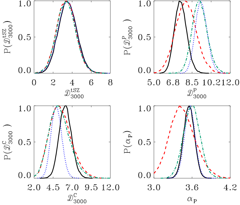
FIG. 9.— 1D likelihood plots of model parameters for different DSFG clustering treatments. Clockwise from top left: the 1D likelihood curves for the amplitudes of the tSZ effect, Poisson DSFG amplitude, Poisson DSFG spectral index and clustered DSFG amplitude. Four cases are plotted for each parameter: The black solid line indicates the baseline model, where \alpha_c = \alpha_p and the power-law clustered template is used. The red dashed line indicates the case where \alpha_c is a free parameter and the power-law clustered template is used. The blue dotted line indicates the case where \alpha_c = \alpha_p and the linear-theory clustered template is used. The blue-green dot-dash line indicates the case where \alpha_c and \alpha_p are independent and the linear-theory clustered template is used. Using the power-law clustered template tends to reduce the power in the Poisson component compared to the linear-theory template. This is expected as the power-law shape has more power at high- \ell than the linear-theory template and the Poisson component also increases with \ell ( D_\ell \propto \ell^2 ). Including an additional free parameter ( \alpha_c ) tends to increase the uncertainty on DSFG-related parameters but not on tSZ.
