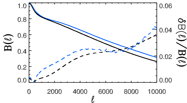
FIG. 1.— Left axis: The measured SPT beam functions at 150 GHz (black line) and 220 GHz (blue line). Right axis: The fractional beam uncertainties at 150 GHz (black dashed line) and 220 GHz (blue dashed line). The beam uncertainty is parametrized by a three component model, the quadrature sum of which is plotted here.
