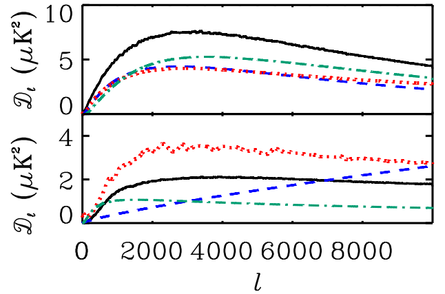
FIG. 5.— Templates used for the tSZ, kSZ, and clustered DSFG power discussed in §6. The top plot shows alternate tSZ templates. The black, solid line is the (baseline) S10 model. The blue, dashed line is the Shaw model. The red, dotted line is the Trac model. The teal dot-dash line is the Battaglia model. The bottom plot shows both kSZ and clustered DSFG templates. The black, solid line is the (baseline) S10 kSZ model. The red, dotted line is the patchy kSZ model. The blue, dashed line is the (baseline) power-law clustered DSFG template. The teal, dot-dash line is the linear-theory clustered DSFG template. The clustered DSFG templates have both been normalized to 1 \mu\text{K}^2 at \ell = 3000 .
