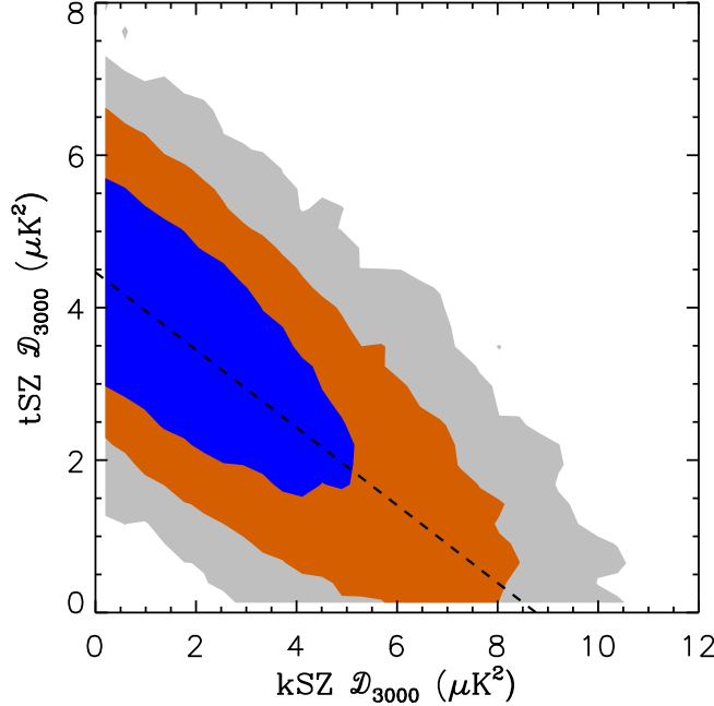
FIG. 8.— 2D likelihood contours for D_{3000}^{tSZ} vs. D_{3000}^{kSZ} . The 68%, 95% and 99.7% contours are marked with blue, orange, and gray respectively. Both tSZ and kSZ model templates are from S10. As in the differenced spectrum analysis, the data primarily constrain a linear combination D_{3000}^{tSZ} + 0.5D_{3000}^{kSZ} = 4.5 \pm 1.0 \mu K^2 . The dashed line shows this axis of near degeneracy. Due to this degeneracy, neither parameter is significantly detected above zero. However, 95% CL upper limits of 5.3 and 6.5 \mu K^2 can be placed on the tSZ and kSZ respectively.
