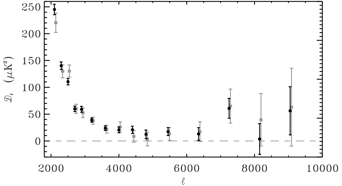
FIG. 13.— The SPT DSFG-subtracted bandpowers from this work ( black circles ) versus the DSFG-subtracted bandpowers presented in L10 ( gray squares ), an earlier reduction of one half of the 2008 data. The damping tail of the primary CMB anisotropy is apparent below \ell = 3000 . Above \ell = 3000 , there is a clear excess due to secondary anisotropies and residual point sources. The two datasets show excellent consistency.
