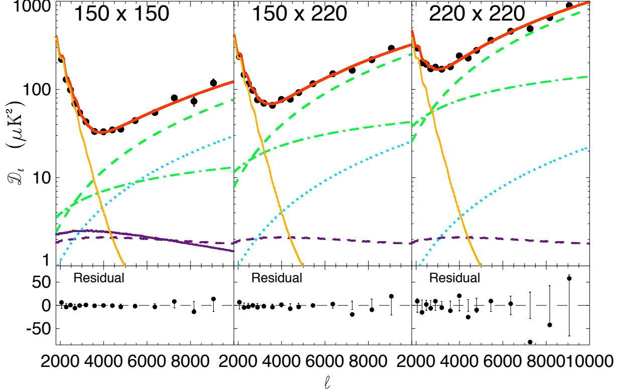
FIG. 3.— Top panel: From left to right, the SPT 150 GHz, 150 × 220 GHz, and 220 GHz bandpowers. Overplotted is the best-fit model (red line) with components shown individually. The lensed primary CMB anisotropy is marked by an orange line. The best-fit tSZ (purple line) and predicted kSZ (purple dashed line) power spectra are also shown. The predicted radio source term is represented by the blue dots. The DSFG Poisson term at each frequency is denoted by the green dashed line and the clustered DSFG component by the green dot-dash line. The damping tail of the primary CMB anisotropy is apparent below \ell = 3000 . Above \ell = 3000 , there is a clear excess with an angular scale dependence consistent with point sources. These sources have low flux (sources detected at > 5\sigma at 150 GHz have been masked) and a rising frequency spectrum, consistent with expectations for DSFGs. Bottom panel: Plot of the residual between the measured bandpowers and best-fit spectrum.
