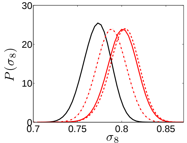
FIG. 16.— \sigma_8 constraints for the S10 ( black line ), Shaw ( red, solid line ), Trac ( red, dashed line ) and Battaglia ( red, dot-dashed line ) models. No model uncertainty has been included.
