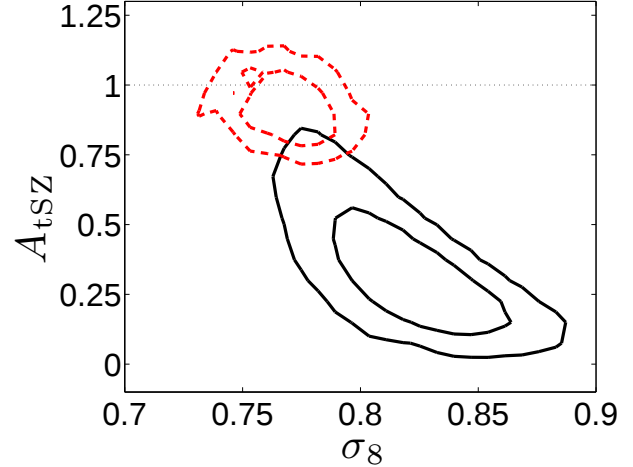
FIG. 15.— 2D likelihood contours at 68% and 95% confidence for \sigma_8 vs. the tSZ scaling parameter A_{\text{tSZ}} (see Eqn. 19). Red, dashed contours show results having resampled the chains applying a lognormal prior to A_{\text{tSZ}} centered at \ln(A_{\text{tSZ}}) = 0 and of width \sigma_{\ln(A_{\text{tSZ}})} = 0.085 . This prior is chosen to reflect the expected sample variance for the observed sky area (see text). Black contours show the results without this prior. All results are for the baseline model (S10 tSZ model and fixed homogeneous kSZ).
