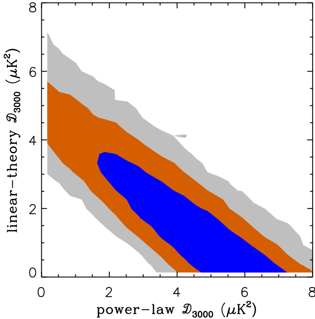
FIG. 10.— 68% (blue), 95% (orange) and 99.7% (grey) likelihood contours for the amplitudes of clustered DSFG components for a model containing both power-law and linear-theory components with independently variable amplitudes. The power-law model is favored at the 1\sigma level; the data do not clearly discriminate between the power-law shape, linear-theory shape, or a linear combination of the two. The choice of clustered DSFG model has no impact on the tSZ power and we adopt the power-law template as the baseline model.
