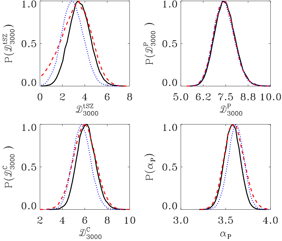
FIG. 7.— 1D likelihood plots for model parameters for three different kSZ treatments. The black, solid line is the baseline (fixed amplitude, S10 homogeneous model) kSZ model. The blue dotted line is the patchy kSZ model with fixed amplitude. The red, dashed line is the model where the amplitude of the (default) kSZ template is free to vary. All powers are measured at \ell = 3000 and 150 GHz. The top left panel shows constraints on the tSZ power spectrum. The preferred tSZ power drops as the assumed kSZ power increases; this trade-off can be seen in more detail in Figure 8. The top right panel shows the likelihood curves for the Poisson DSFG power, and the bottom left panel shows the same for the clustered DSFG power. The bottom right panel shows the Poisson DSFG spectral index. There is a slight decrease in clustered DSFG power with the increased kSZ power expected from patchy reionization; this is accompanied by small shift to higher spectral indices, preserving the higher-frequency bandpowers.
