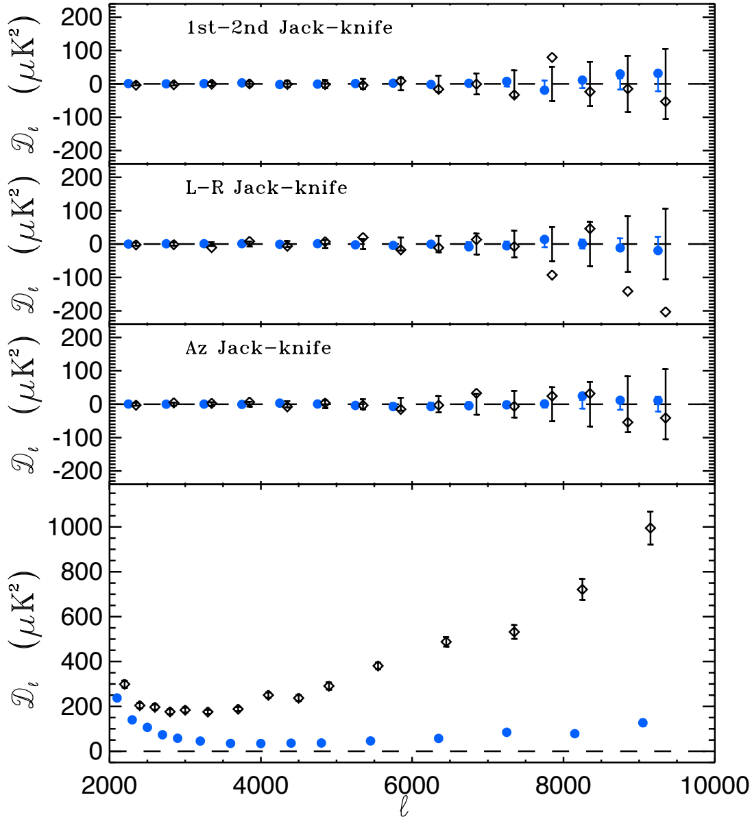
FIG. 2.— Jackknives for the SPT data set at 150 GHz (blue circles) and 220 GHz (black diamonds). For clarity, the 220 GHz jackknives have been shifted to the right by \Delta\ell = 100 . Top panel: Bandpowers of the “first half - second half” jackknife compared to the expected error bars about zero signal. Disagreement with zero would indicate either a noise misestimate or a time-dependent systematic signal. Second panel: Power spectrum of the left-going minus right-going difference map. This test yields strong constraints on the accuracy of the detector transfer function deconvolution and on possible directional systematics. Third panel: Bandpowers for the difference map when the data are split based on the observed very large scale ( \ell < 100 ) ground pickup as a function of azimuth. Signals fixed in azimuth, such as ground pickup on smaller scales, would produce non-zero power. We see no evidence for ground-based pickup across this \ell -range. The cumulative probability to exceed the \chi^2 observed in these three tests at 150 and 220 GHz is 55%. Bottom panel: The un-differenced SPT power spectra at each frequency for comparison.
