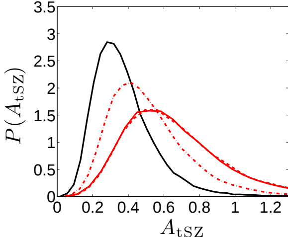
FIG. 14.— Posterior distribution of the tSZ scaling parameter A_{\text{tSZ}} (see Equation 19 and Table 6) for each of the tSZ templates. The black line shows the S10 prediction. The red solid, dashed and dot-dashed lines show the results for the Shaw, Trac, and Battaglia models, respectively. As expected, the preferred value of A_{\text{tSZ}} increases for models which predict less tSZ power. Note that a value of A_{\text{tSZ}} = 1 would demonstrate consistency between the predicted and observed tSZ power.
