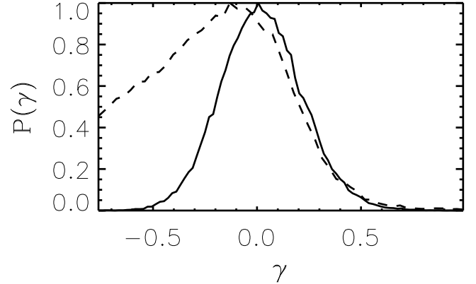
FIG. 11.— The 1D likelihood curve for the tSZ-DSFG correlation factor, \gamma . The linear-theory clustered DSFG template and the S10 tSZ template are assumed. The solid line indicates the case where the kSZ amplitude is held fixed. The data favor no correlation albeit with significant uncertainty. The dashed line denotes the likelihood curve when the kSZ amplitude is allowed to vary. The data remain consistent with zero correlation, but large negative correlations become possible. Essentially, the kSZ power increases to balance the lower predicted power due to anti-correlation. Because the tSZ and kSZ amplitudes are highly correlated, additional kSZ power reduces the apparent tSZ power.
