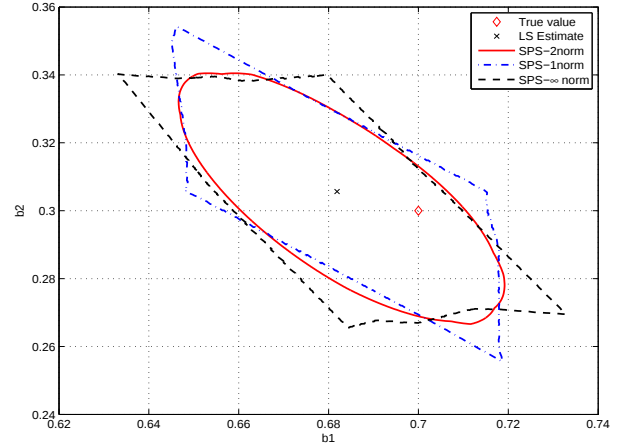
Figure 3. 95% confidence regions using various norms, n = 400 , m = 100 .
