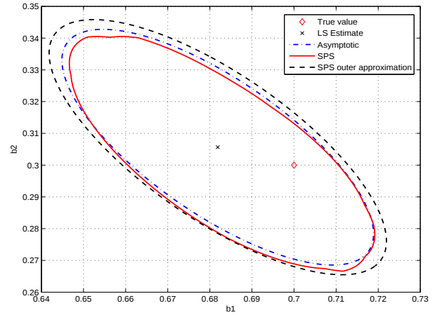
Figure 2. 95% confidence regions, n = 400 , m = 100 .
