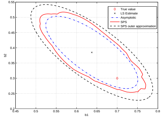
Figure 1. 95% confidence regions, n = 25 , m = 100 .
