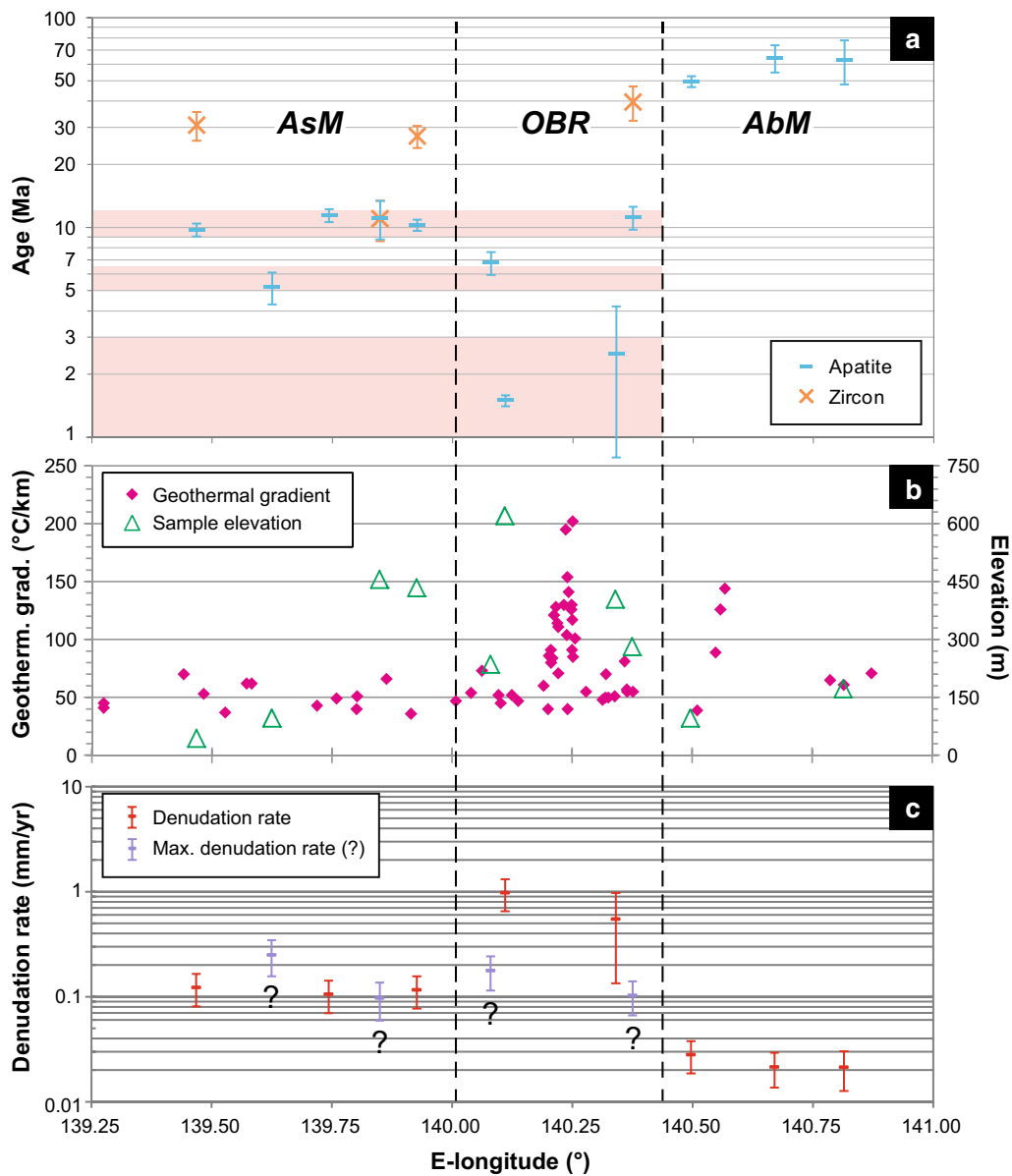
Fig. 4 a Longitude versus (U–Th)/He age. The weighted mean ages \pm 95\% confidence intervals are shown. The light pink bands indicate approximate range of timing of the three major recent uplift episodes of the NE Japan Arc in 12–9 Ma, 6.5–5 Ma, and after 3 Ma (e.g., Nakajima et al. 2006; Fujiwara et al. 2008; Moriya et al. 2008). b Longitude versus geothermal gradient and sample elevation. Geothermal gradient data of 37.5°N–38.5°N from Tanaka et al. (2004) are plotted. c Mean denudation rates calculated from AHe ages. Purpuric data shown with “?” indicate less reliable denudation rates which might reflect reheating related to magmatism; the computed denudation rates are thought to indicate the maximum value
