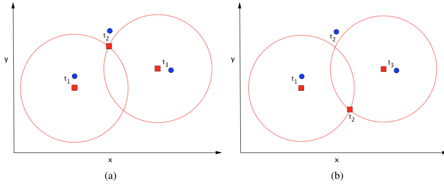
Fig. 5 Illustration of two trajectories T^1 and T^2 in space dimensions (time dimension is shown as label) (a) the minimum possible distance and (b) the maximum possible distance of the trajectories in Fig. 4(a) at time t_2
