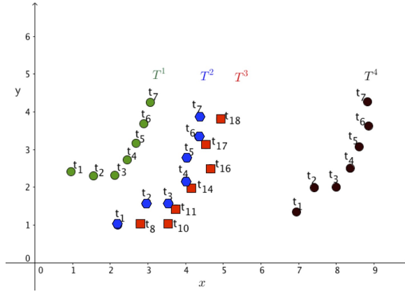
Fig. 3 Illustration of four different spatiotemporal trajectories. T^2 is more similar to T^4 in terms of speed and bearing changes, to T^3 in terms of spatial similarity and to T^1 concerning spatiotemporal similarity
