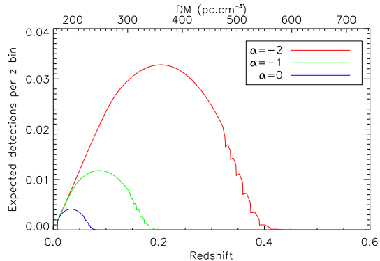
Fig. 1.— Predicted distribution of FRB detections in redshift for each spectral index and a 10.5 hour observation. The structure in the curves at the high redshift/DM end is due to the sensitivity contribution of the sidelobes of the MWA tile beam, as described in Trott, Tingay & Wayth (2013).
