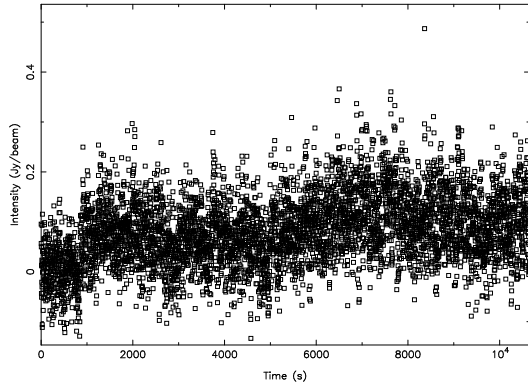
Fig. 5.— An example de-dispersed time series for pixel (513,138) (from data in Figure 4) in which a 6\sigma event was detected at DM=594.08 \text{ pc cm}^{-3} , 8364 s from the start of the observation.
