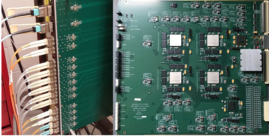
Figure 17. The physical RTM (left) and MAIN Second Stage Boards (right).
