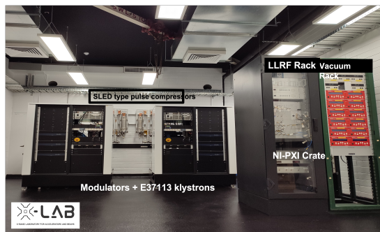
Figure 1. Layout of the new X-LAB and the configuration of the Mel-BOX test stands.
