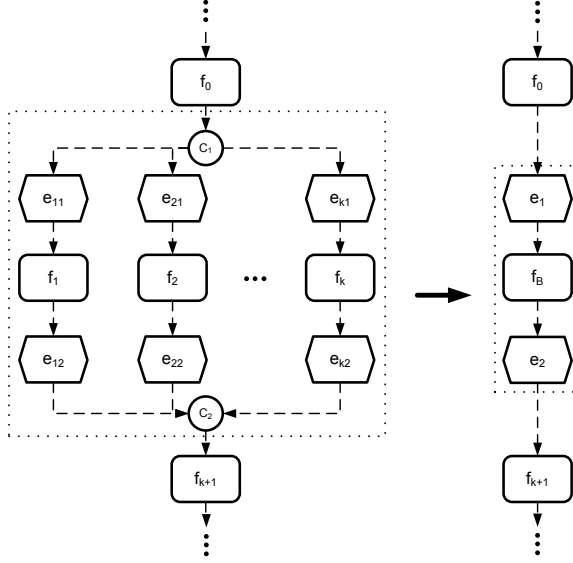
Fig. 1.4. Block abstraction
