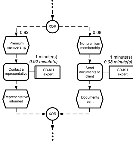
Fig. 1.1. Example of the EPC fragment enriched with probabilities and efforts
