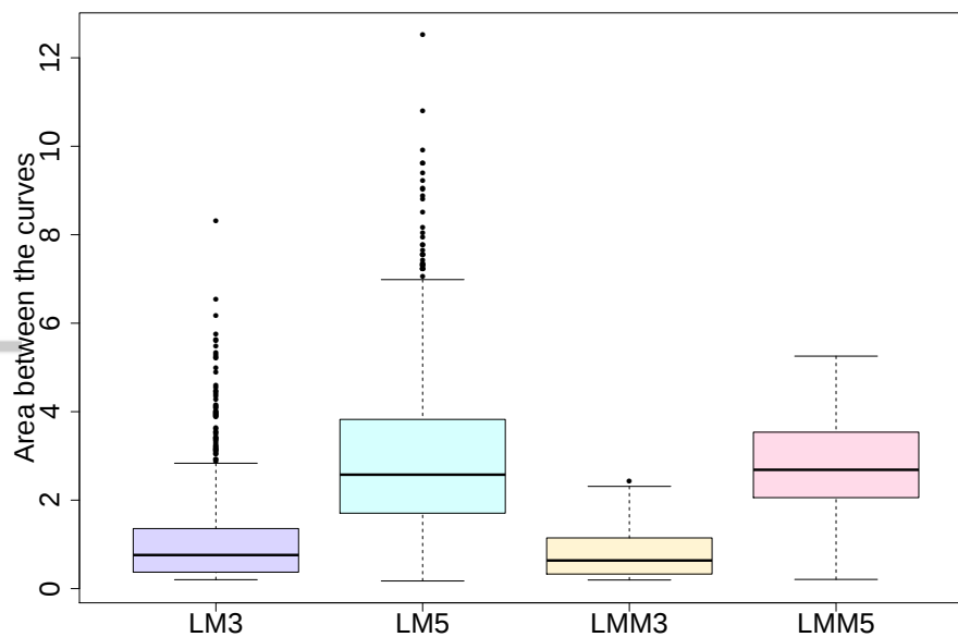
Figure 4. Boxplots displaying the range of values for the area between the population average and estimated predictions curves for the four models.
