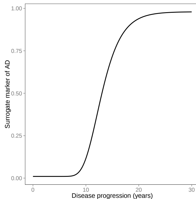
Figure 2. An example of a 5PL curve modelled over 30 years for a surrogate marker of AD. The following parameter values are utilised for this figure: b = 13 , a = 0.4 , c = 0.01 , f = 0.98 , and g = 20
