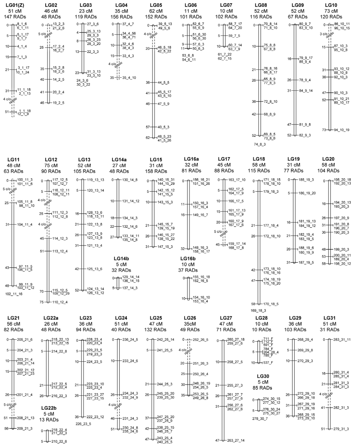
Figure 2. Linkage map of the Plutella xylostella (n=31) genome. This was inferred from 2,878 RAD alleles collapsed into 285 discrete RAD markers. Each linkage group contains between 10 and 158 RAD alleles (labelled RADs) and the total map length is 1,292 cM. Each RAD marker is labelled with three numbers (i, ii, iii) corresponding to (i) the RAD marker (1–285), (ii) the chromosome number (1–31) and (iii) the number of RAD alleles at that marker. Linkage groups 1–28 are homologous to the B. mori (n=28) chromosome numbering system, and LG29, LG30 and LG31 represent fusions to chromosomes 11, 23 and 24 respectively in B. mori . Dashed lines represent manual linkages inferred from 3, 4 or 5 genotype differences that were otherwise left ungrouped due to small sample size. As 20 progeny were used to construct the map, distances were approximated as 5 cM (1/20) per 1 crossing-over (c/o) event. On chromosomes 14, 16 and 22, markers formed two distinct groups and may be separated by regions of high recombination rates or chromosomal assignment error. In total, 11 of the 285 RAD markers could not be confidently assigned to their predicted chromosome. Linkage group 28 contained only four RAD markers at a single locus. Six additional markers were identified for this chromosome using JoinMap 3.0, from the remaining paternal markers not assigned to linkage groups. doi:10.1371/journal.pone.0019315.g002
