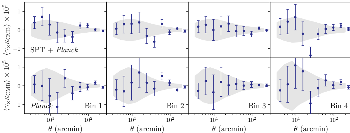
FIG. 15. Cross-correlation between than cross-component of shear with CMB lensing for the SPT+ Planck field (top) and the Planck field (bottom) and for different redshift bins. The grey band shows the statistical uncertainties for \langle\gamma_t\kappa_{\text{CMB}}\rangle .
