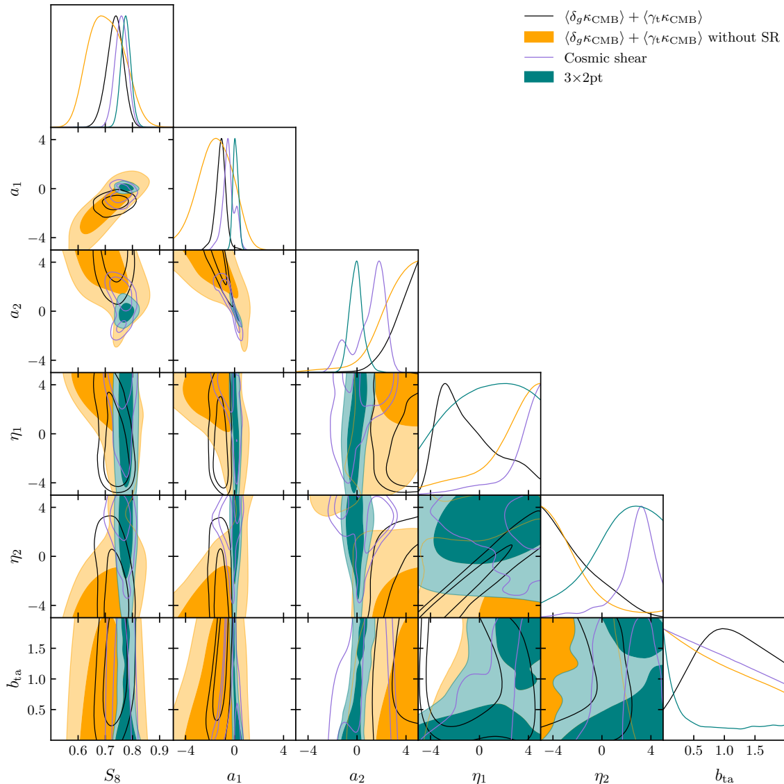
FIG. 6. Constraints on S_8 and the IA parameters from our fiducial \langle \delta_g \kappa_{\text{CMB}} \rangle + \langle \gamma_t \kappa_{\text{CMB}} \rangle results, cosmic shear and 3 \times 2\text{pt} . We also include the \langle \delta_g \kappa_{\text{CMB}} \rangle + \langle \gamma_t \kappa_{\text{CMB}} \rangle constraints without the lensing ratio (SR) likelihood for comparison.
