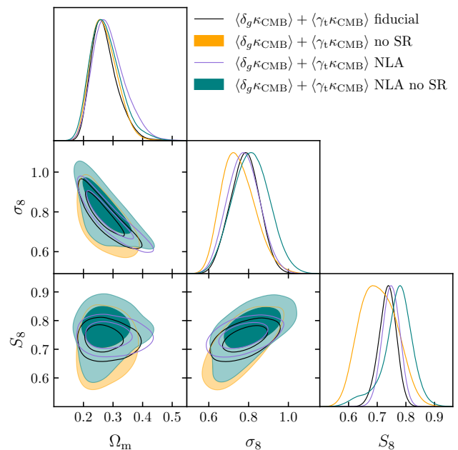
FIG. 5. Constraints on cosmological parameters \Omega_m, \sigma_8 , and S_8 using the \langle\delta_g\kappa_{\text{CMB}}\rangle + \langle\gamma_t\kappa_{\text{CMB}}\rangle probes with and without including the lensing ratio (SR) likelihood, and when assuming the NLA IA model instead of our fiducial IA model TATT.
