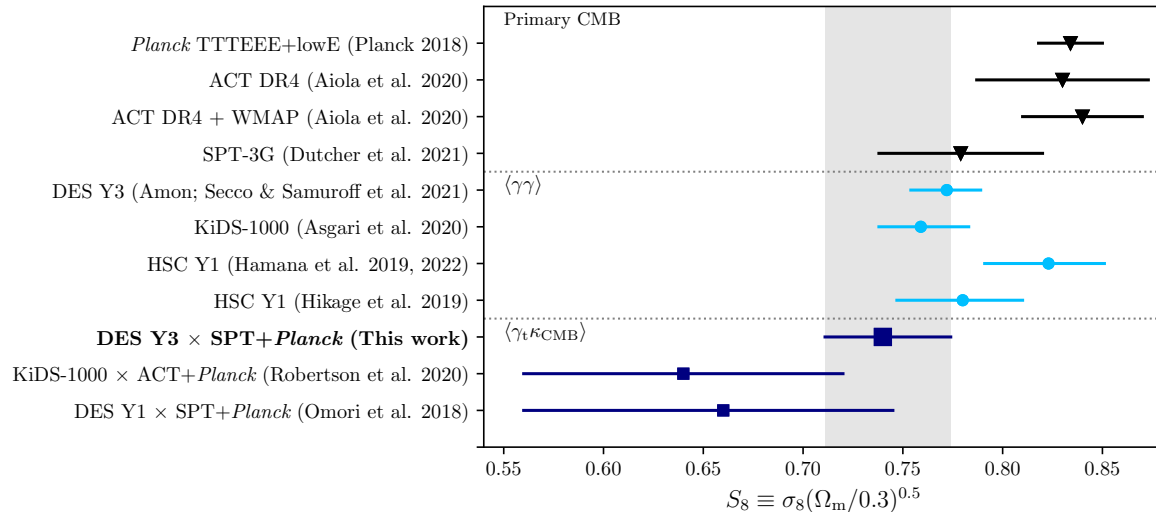
FIG. 10. Comparison of late-time measurements of S_8 from lensing-only data (cosmic shear \langle\gamma\gamma\rangle ) and galaxy shear-CMB lensing cross-correlation \langle\gamma_t\kappa_{\text{CMB}}\rangle ) to the inferred value of S_8 from the primary CMB.
