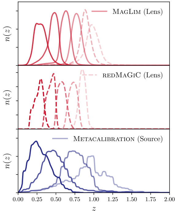
FIG. 1. Redshift distribution for the tomographic bins for the galaxy samples used in this work: the MAGLIM lens sample (top), the REDMAGIC lens sample (middle) and the METACALIBRATION source sample (bottom). The fiducial lens sample only uses the first four bins of the MAGLIM sample, or the solid lines. We perform tests with the non-fiducial samples (dashed lines) for diagnostic purposes.
