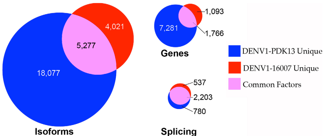
Figure 2. Comparison of differential regulation of genes, isoforms and splicing in DENV1-16007 and DENV1-PDK13. doi:10.1371/journal.pntd.0002107.g002
