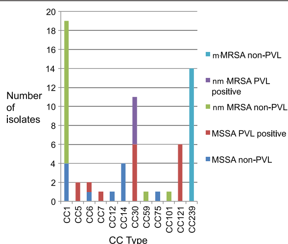
Figure 2 Clonal complex types of S. aureus isolated from patients at CWMH, Fiji. Clonal complexes identified from SNP typing of Staphylococcus aureus isolates collected from the Colonial War Memorial Hospital, Fiji (MSSA: methicillin sensitive Staphylococcus aureus ; nmMRSA: non-multidrug-resistant methicillin resistant Staphylococcus aureus ; mMRSA: multidrug-resistant MRSA; PVL: Pantone Valentine Leukocidin).
