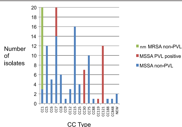
Figure 1 Clonal complex types of S. aureus isolated from Fijian schoolchildren's impetigo lesions. Clonal complexes identified from SNP-typing of Staphylococcus aureus isolates collected from impetigo lesions in school children in Fiji (MSSA: methicillin sensitive Staphylococcus aureus ; nmMRSA: non-multidrug-resistant methicillin resistant Staphylococcus aureus ; PVL: Pantone Valentine Leukocidin).
