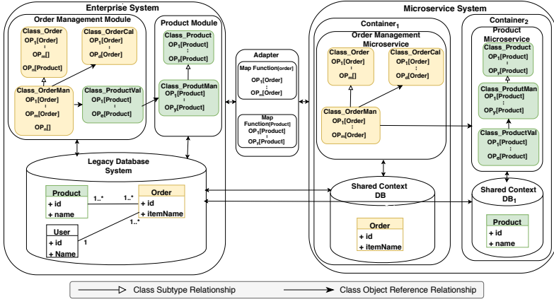
Fig. 1: Overview of an enterprise system extended with extracted microservices.
