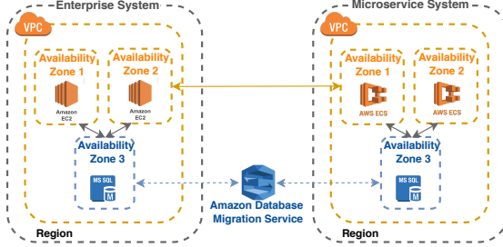
Fig. 4: System implementation in AWS.
