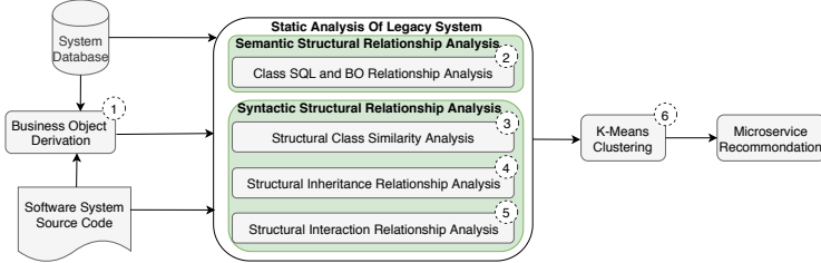
Fig. 2: Overview of our microservice discovery approach.
