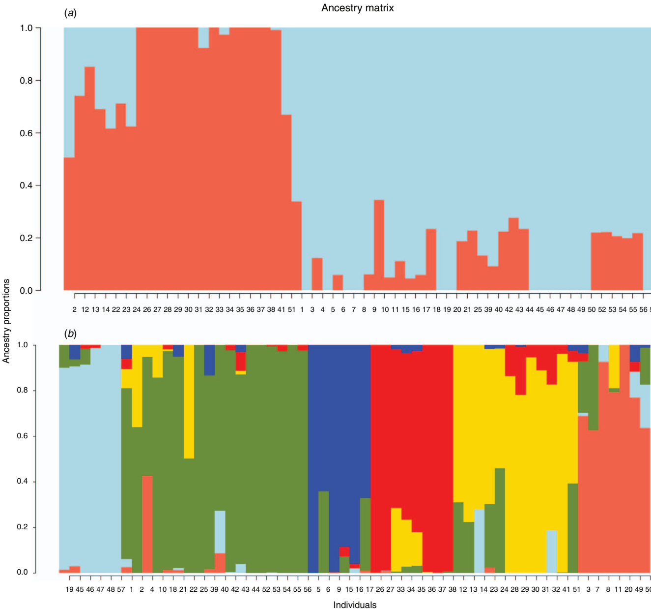
Fig. 3. Q-plots showing clustering of 57 wild phalaris accessions based on analysis of genotypic data by using admixture analysis for: (a) K = 2 , and (b) K = 6 . Each accession is represented by a vertical bar. The proportion of each bar that is of a specific colour indicates the probability that the individual belongs to the cluster of that colour. Cultivar names and corresponding individual numbers (1–57) as shown on the x-axis are provided in Appendix 2.
