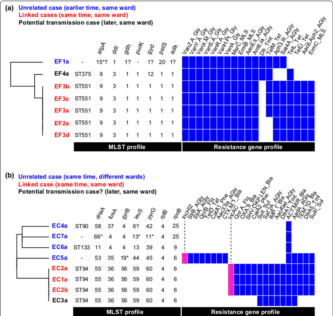
Figure 8 SRST2 analysis of hospital outbreak investigation. (a) Isolate genetic profiles obtained from SRST2 analysis, indicating that case EF4 was distinct in both sequence type and resistance gene profile from the outbreak cases EF2 and EF3. Full WGS analysis showed a similar result [15]. (b) Isolate genetic profiles obtained from SRST2 analysis, including plasmid replicons detected (pink). The profiles indicate that case EC3 shared the same sequence type as the linked cases EC1 and EC2 (ST94), but lacked the IncA/C plasmid and had a distinct resistance gene profile. Full WGS analysis showed that EC1 and EC2 isolates were much closer to each other ( \leq 22 SNPs) than to EC3 ( > 150 SNPs) [15].
