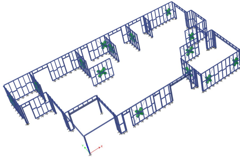
a) One-storey building (Amalfi)
