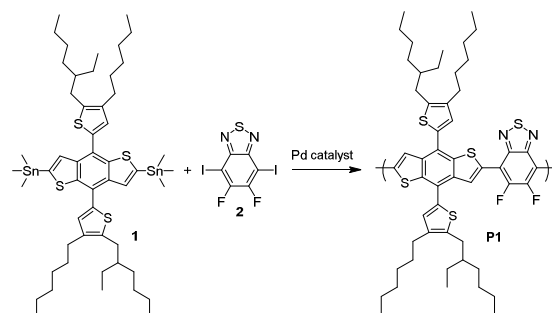
65 Fig. 1 Chemical structures of compound 1 and 2 and the Stille polymerization for conjugated polymer P1.
