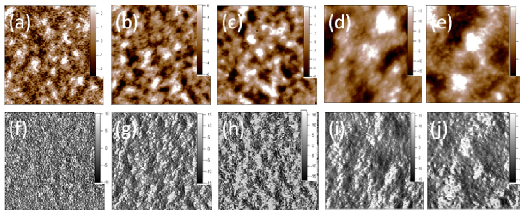
Fig. 4 AFM images of PI/PC 71 BM (1:2 weight ratio) films. (a) and (f) PI-9.6K/PC 71 BM ; (b) and (g) PI-17.1K/PC 71 BM ; (c) and (h), PI-32.0K/PC 71 BM ; (d) and (i) PI-72.9K/PC 71 BM ; (e) and (j) PI-138.9K/PC 71 BM . (a)-(e) are height images; (f)-(j) are phase images. All images are 2 \times 2 \mu\text{m} .
