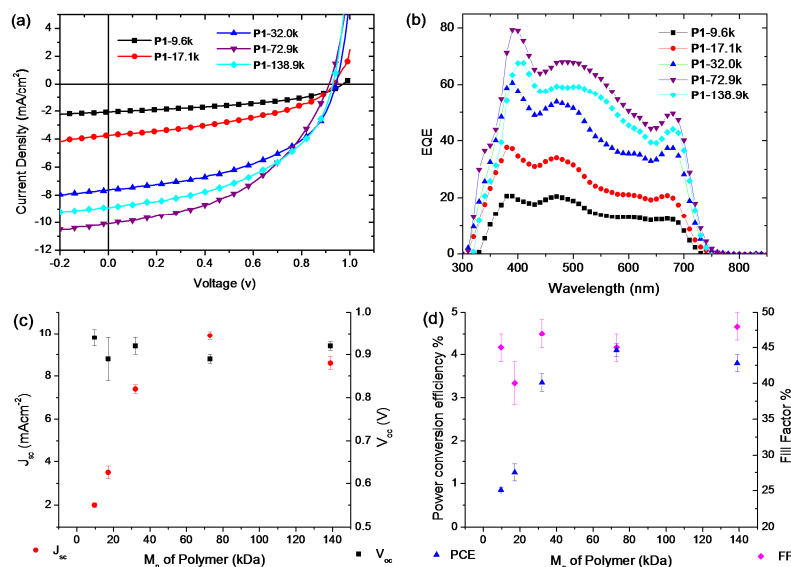
Fig. 3 (a) J - V characteristics of photovoltaic devices fabricated with different molecular weight P1 / PC_{71}BM under AM 1.5G irradiation ( 100 \text{ mW cm}^{-2} ). (b) EQE curves of the BHJ solar cells fabricated under the same optimized conditions as used for the J - V measurements. (c) M_n of polymer plotted against J_{sc} and V_{oc} and (d) M_n of polymer plotted against FF and PCE.
