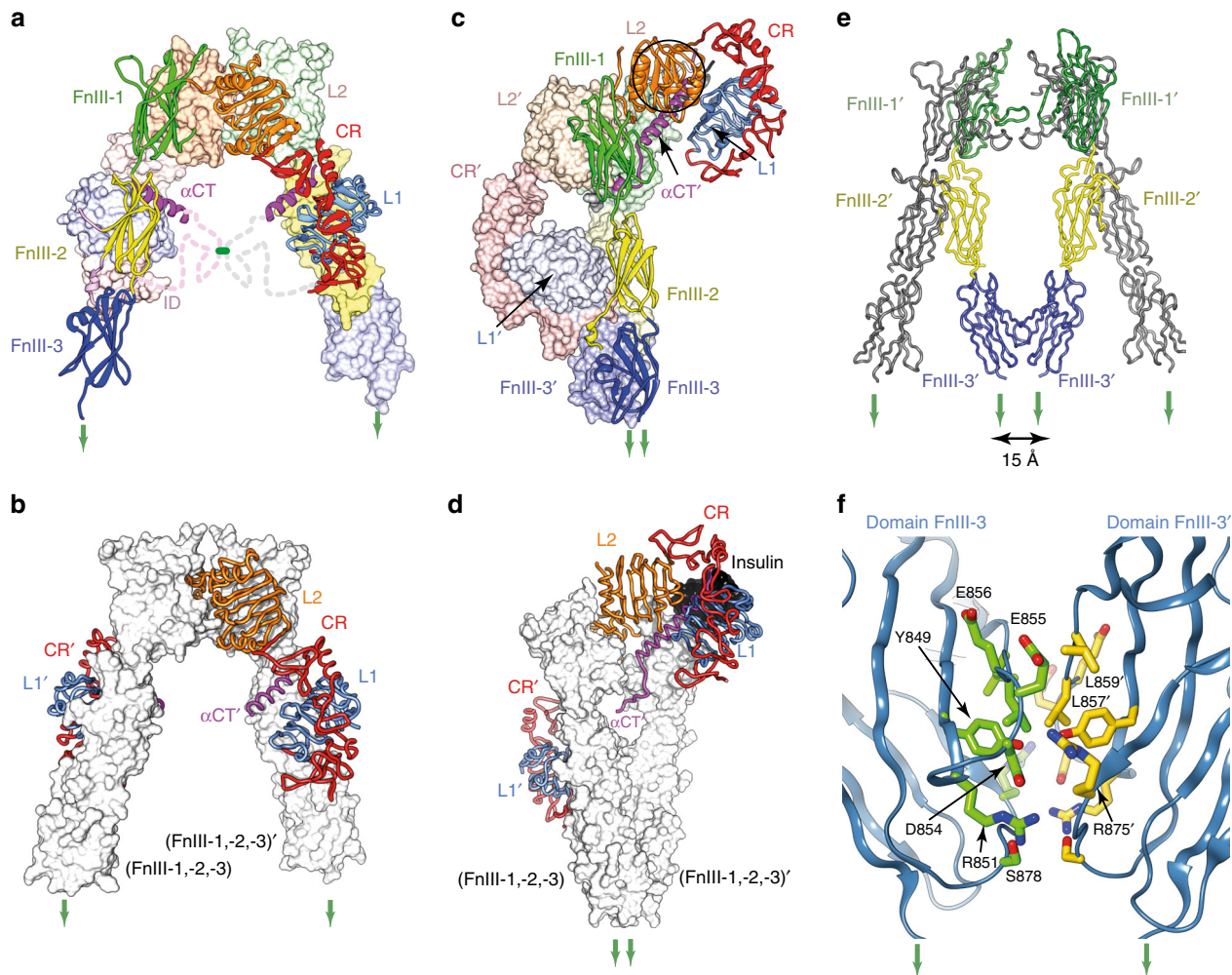
Fig. 2 Comparison of the cryo-EM structure of IR \Delta\beta -ziplnsFv with the crystal structure of apo IR \Delta\beta . a Domain arrangement in apo IR \Delta\beta (left) with domains colored as in Fig. 1a. b Apo IR \Delta\beta but with only domains L1, CR, L2, L1', CR', and \alpha CT' shown in color (for comparison with panel (d)). c Domain arrangement in IR \Delta\beta -ziplnsFv with domains colored as in Fig. 1a. d IR \Delta\beta -ziplnsFv but with only domains L1, CR, L2, L1', CR', and \alpha CT' shown in color in order to highlight the rearrangement of the insulin-bound (L1-CR-L2) + \alpha CT' module with respect to apo IR \Delta\beta (panel (b)). e Comparison of the relative disposition of domains FnIII and FnIII' in apo IR \Delta\beta (grey) and in IR \Delta\beta -ziplnsFv (colored). f Pseudo-two-fold-symmetric interaction of domains FnIII-3 and FnIII-3' within IR \Delta\beta -ziplnsFv. For clarity, only one member of each pseudo-symmetry-related residue pair is labeled. Green arrows in all panels indicate the direction of membrane entry. Panel (a) is adapted from Fig. 1a of Xu et al. 22
