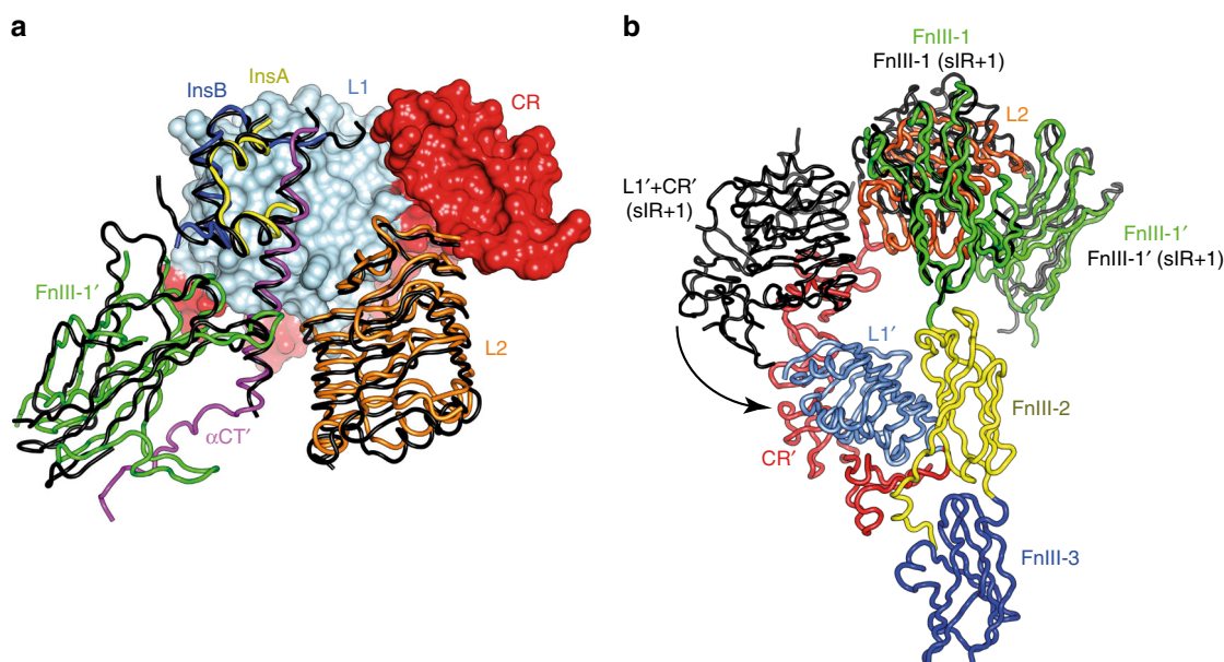
Fig. 4 Comparison of the cryo-EM structure of IR \Delta\beta -ziplnsFv with the insulin-complexed cryo-EM structures sIR + 2 and sIR + 1 7 . a Schematic illustrating the similar environments of insulin, based on an overlay of the common L1-CR modules of IR \Delta\beta -ziplnsFv and sIR + 2 (shown as surface for IR \Delta\beta -ziplnsFv and omitted for sIR + 2). Remaining domains are shown as colored coil for IR \Delta\beta -ziplnsFv and black coil for sIR + 2. b Schematic illustrating the altered disposition of the respective unliganded L1-CR modules in IR \Delta\beta -ziplnsFv and in sIR + 1. Overlay is based on common FnIII-1/FnIII-1' modules. Domains are shown as colored coil for IR \Delta\beta -ziplnsFv and black coil for sIR + 1
