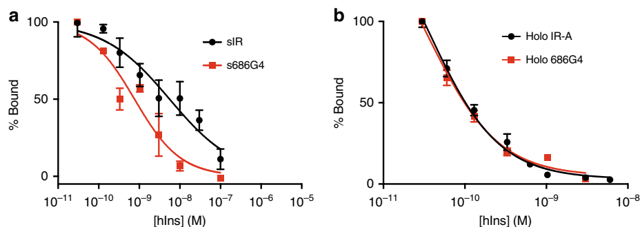
Fig. 5 Insulin competition-binding assays for 686G4 IR mutants. a Insulin competition-binding assay of sIR ( IC_{50} = 5.6 \pm 1.7 nM; n = 4 technical replicates per concentration point) and s686G4 ( IC_{50} = 0.76 \pm 0.16 nM; n = 4 technical replicates per concentration point). The IC_{50} values differ at the 95% level of confidence based on an F test ( P < 0.0001 ; no. of degrees of freedom = 54; two individual measurements of sIR affinity were judged as systematically in error and omitted from the analysis). b Insulin competition-binding assay of hIR-A ( IC_{50} = 52 \pm 10 pM; n = 4 technical replicates per data point) and holo 686G4 ( IC_{50} = 30 \pm 6 pM; n = 10 technical replicates per data point). The IC_{50} values are the same at the 95% level of confidence based on an F test ( P = 0.084 ; no. of degrees of freedom = 86). In both ( a ) and ( b ), error bars reflect s.e.m. and are not shown when smaller than marker size
