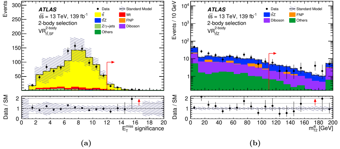
Figure 3. Two-body selection. Distributions of the E_T^{\text{miss}} significance in (a) \text{VR}_{t\bar{t},\text{SF}}^{2\text{-body}} and (b) m_{T2}^{4\ell} in \text{VR}_{t\ell Z}^{2\text{-body}} , each after the background fit. The contributions from all SM backgrounds are shown as a histogram stack. “Others” includes contributions from VVV , t\bar{t}t , t\bar{t}t\bar{t} , t\bar{t}W , t\bar{t}WW , t\bar{t}WZ , t\bar{t}H , and tZ processes. The hatched bands represent the total statistical and detector-related systematic uncertainty. The rightmost bin of each plot includes overflow events. In the upper panels, red arrows indicate the validation region selection criteria. The bottom panels show the ratio of the observed data to the total SM background prediction, with hatched bands representing the total uncertainty in the background prediction; red arrows show data outside the vertical-axis range.
