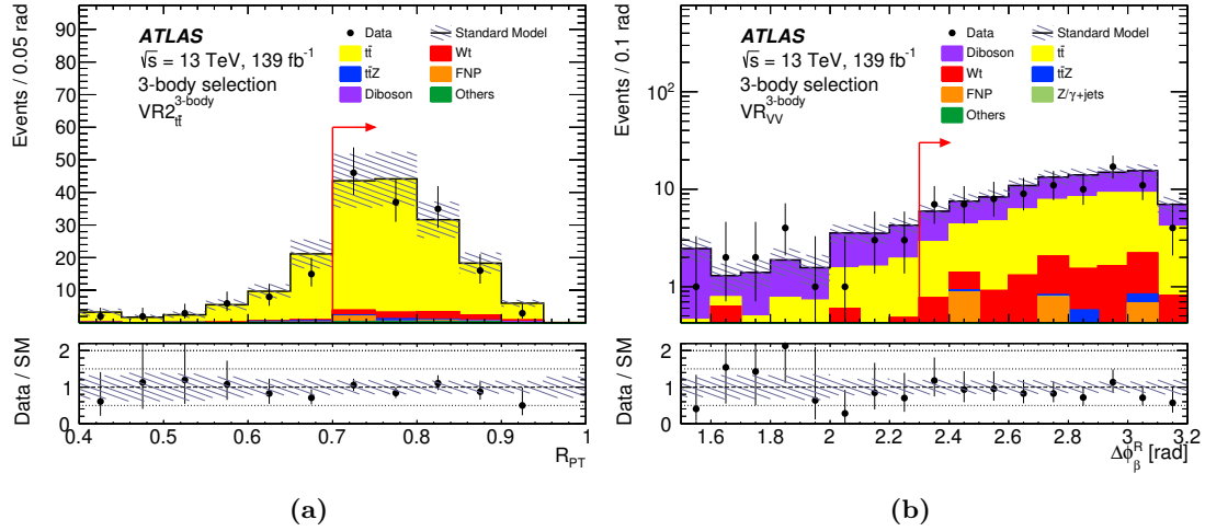
Figure 5. Three-body selection. Distributions of (a) R_{p_T} in the validation region \text{VR}(2)_{t\bar{t}}^{3\text{-body}} and (b) \Delta\phi_\beta^R in the validation region \text{VR}_{VV}^{3\text{-body}} , after the background fit. The contributions from all SM backgrounds are shown as a histogram stack. “Others” includes contributions from VVV , t\bar{t}t , t\bar{t}t\bar{t} , t\bar{t}W , t\bar{t}WW , t\bar{t}WZ , t\bar{t}H , and tZ processes. The hatched bands represent the total statistical and detector-related systematic uncertainty. The bottom panels show the ratio of the observed data to the total SM background prediction, with hatched bands representing the total uncertainty in the background prediction.
