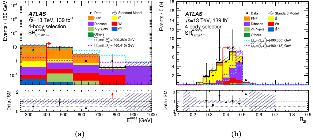
Figure 13. Four-body selection. (a) distributions of E_T^{\text{miss}} in \text{SR}_{\text{4-body}}^{\text{Small } \Delta m} and (b) distribution of R_{2l4j} in \text{SR}_{\text{4-body}}^{\text{Large } \Delta m} for events satisfying the selection criteria of the given SR, except the one for the presented variable, after the background fit. The contributions from all SM backgrounds are shown as a histogram stack. “Others” includes contributions from VVV , t\bar{t}t , t\bar{t}t\bar{t} , t\bar{t}W , t\bar{t}WW , t\bar{t}WZ , t\bar{t}H , and tZ processes. The hatched bands represent the total statistical and systematic uncertainty. The rightmost bin of each plot includes overflow events. Reference top squark pair production signal models are overlayed for comparison. Red arrows in the upper panel indicate the signal region selection criteria. The bottom panels show the ratio of the observed data to the total SM background prediction, with hatched bands representing the total uncertainty in the background prediction; red arrows show data outside the vertical-axis range.
