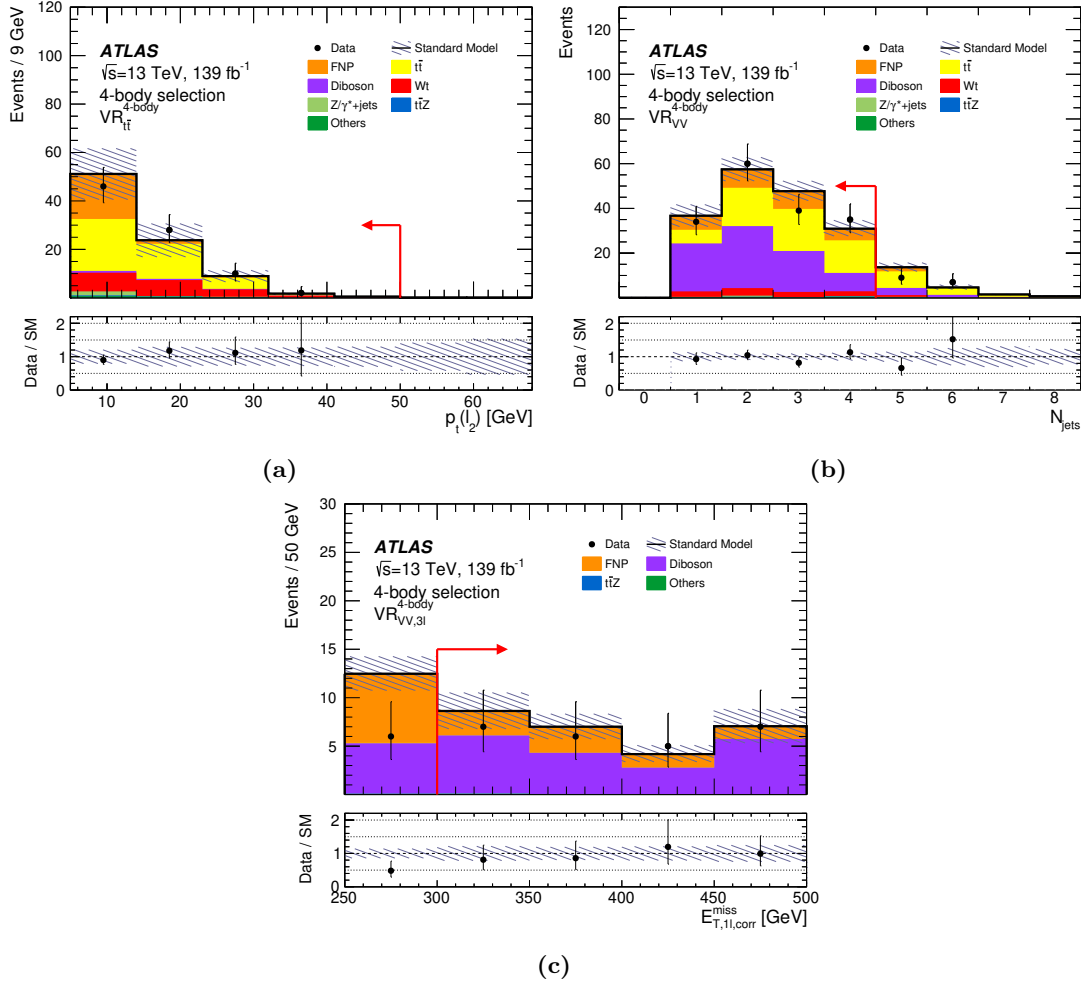
Figure 7. Four-body selection. Distributions of (a) p_T(\ell_2) in VR_{t\bar{t}}^{4-body} , (b) n_{jets} in VR_{VV}^{4-body} and (c) E_{T,1\ell,corr}^{miss} in VR_{VV,3\ell}^{4-body} after the background fit. The contributions from all SM backgrounds are shown as a histogram stack. “Others” includes contributions from VVV , t\bar{t}t , t\bar{t}t\bar{t} , t\bar{t}W , t\bar{t}WW , t\bar{t}WZ , t\bar{t}H , and t\bar{t}Z processes. The hatched bands represent the total statistical and detector-related systematic uncertainty. The rightmost bin of each plot includes overflow events. In the upper panels, red arrows indicate the validation region selection criteria. The bottom panels show the ratio of the observed data to the total SM background prediction, with hatched bands representing the total uncertainty in the background prediction.
