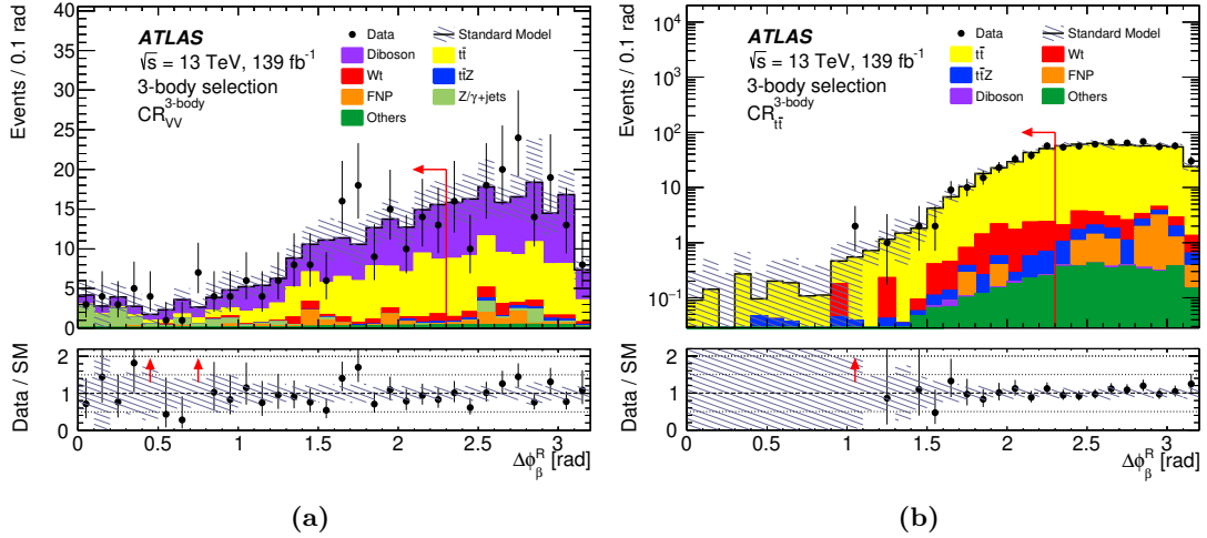
Figure 4. Three-body selection. Distributions of (a) \Delta\phi_{\beta}^R in the CR_{VV}^{3\text{-body}} selection, and (b) in the CR_{tt}^{3\text{-body}} selection, after the background fit. The contributions from all SM backgrounds are shown as a histogram stack. “Others” includes contributions from VVV , t\bar{t}t , t\bar{t}t\bar{t} , t\bar{t}W , t\bar{t}WW , t\bar{t}WZ , t\bar{t}H , and tZ processes. The hatched bands represent the total statistical and detector-related systematic uncertainty. In the upper panels, red arrows indicate the control region selection criteria. The bottom panels show the ratio of the observed data to the total SM background prediction, with hatched bands representing the total uncertainty in the background prediction; red arrows show data outside the vertical-axis range.
