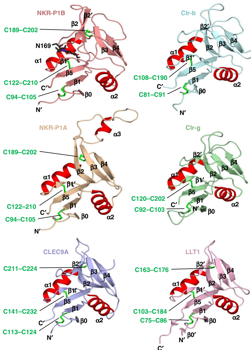
Fig. 1 The CTLD fold of NKR-P1B and Clr-b. Comparison of the structures of NKR-P1B and Clr-b with other related receptors and ligands including mouse NKR-P1A (PDB ID: 3M9Z), Clr-g (PDB ID: 3R51), CLEC9A (PDB ID: 3VPP) and LLT1 (PDB ID 4QKG). \alpha -helices are shown in red and disulfide bonds are represented as green sticks. The single GlcNAc moiety attached to Asn169 of NKR-P1B is shown as black sticks
