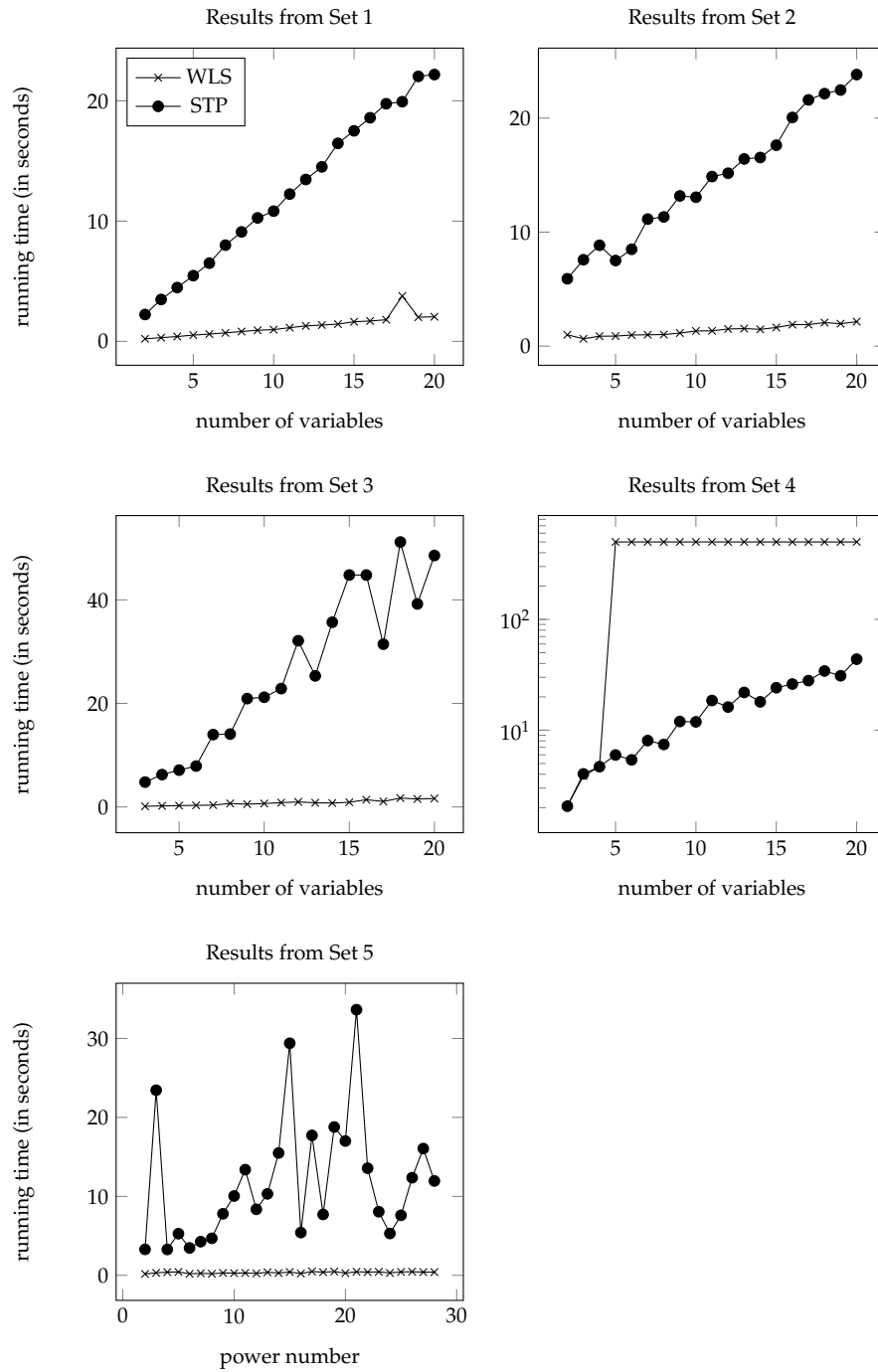
Fig. 4 Word-level solver vs STP on multiplication constraints evaluation
