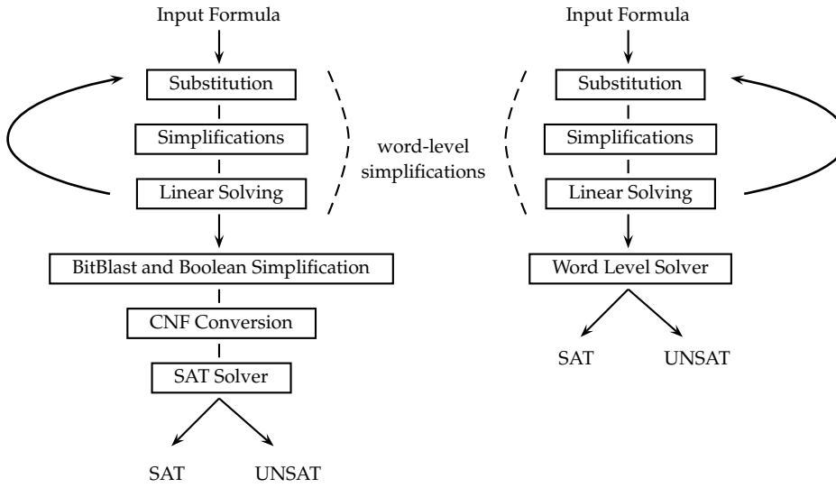
Fig. 2 The main structure of STP (left) and word-level solvers (right)
