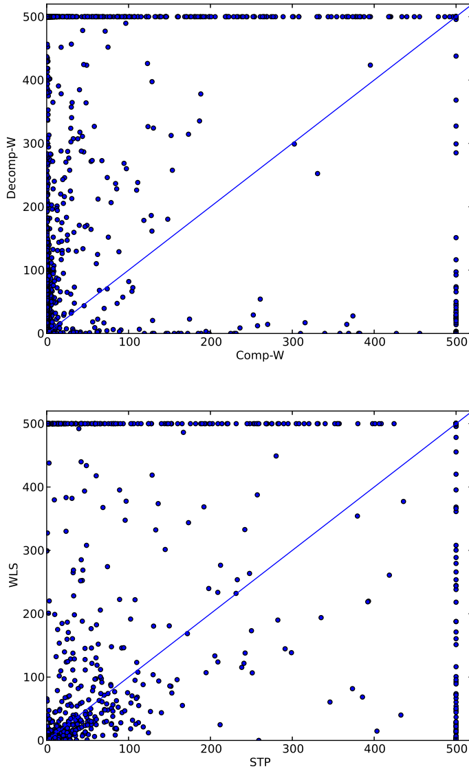
Fig. 3 Comp-W vs Decomp-W (top) and STP vs WLS (bottom)
