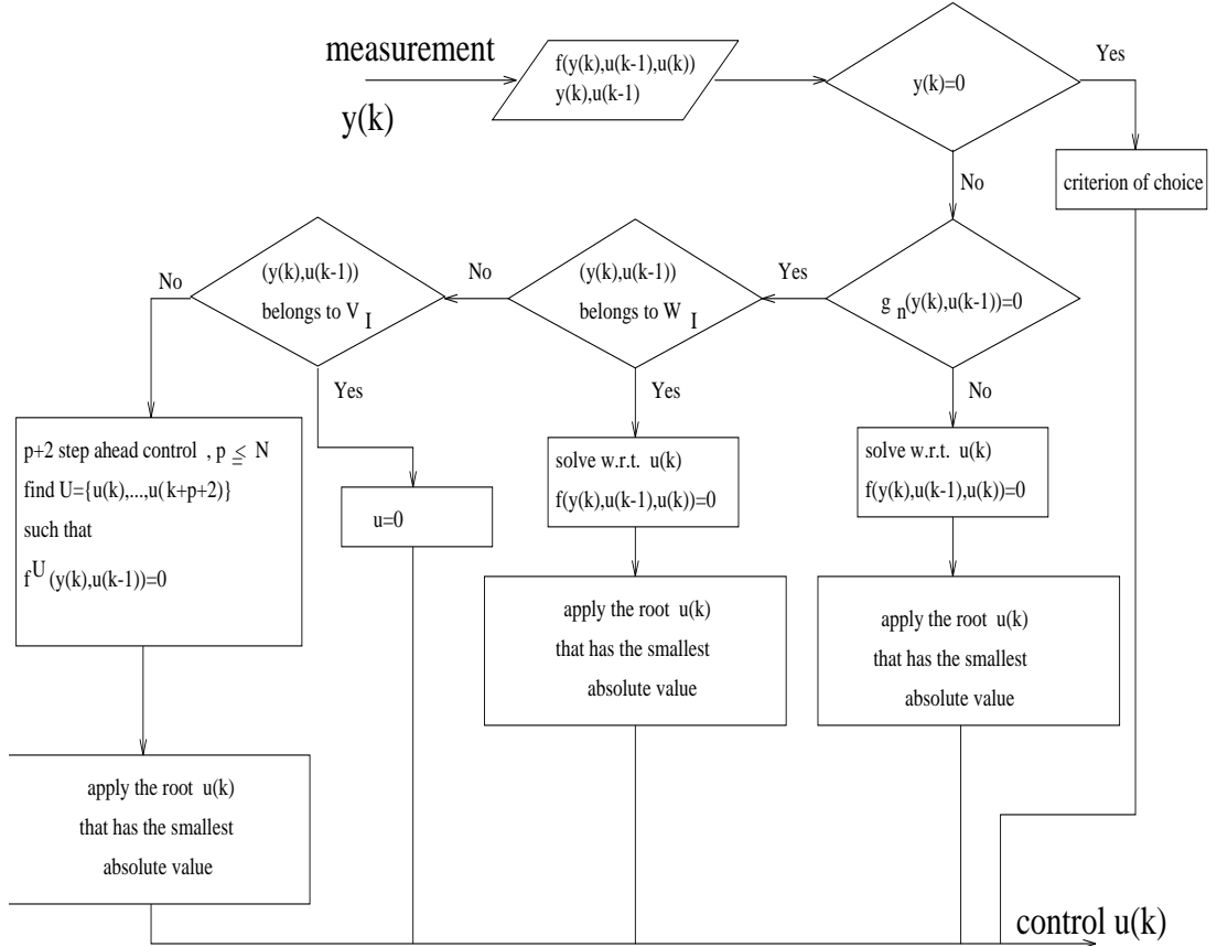
FIG. 1. Output dead beat controller - algorithm
