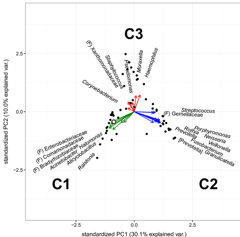
Fig 3. Principle component analysis (PCA) of the 23 most abundant taxa delineates three distinct bacterial associations or cluster types. Scaled PCA of the 23 most abundant taxa (representing \geq 0.5\% of the average relative abundance), for all RML samples and the average background community (white circle). Vector length and direction indicate the relative contribution of each taxon. Three associative groups of taxa are apparent. These clusters types can be summarized as background signal (C1, green), oral-like (C2, blue), or pathogen (C3, red) communities.
