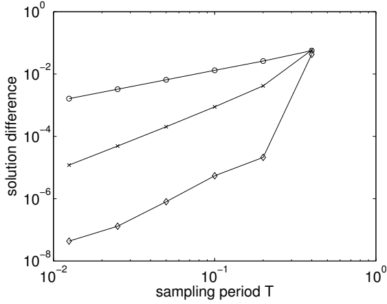
Fig. 5.2. Difference between continuous time and sampled-data solutions at t = 1 for sampled-data controllers (5.1, o), (5.2, x) and (5.3, ◊)
