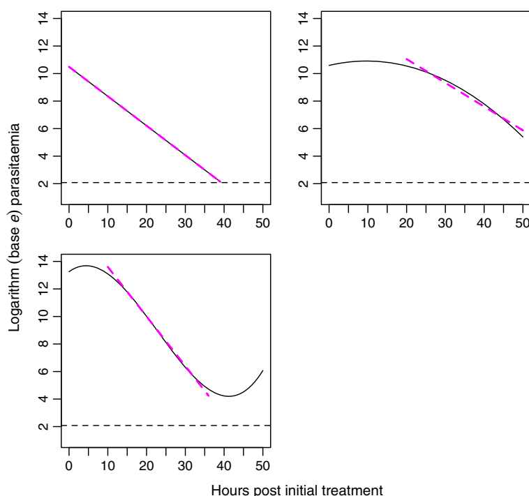
Figure 1 Graphical representation of the Parasite Clearance Estimator. The black lines represent typical log parasitaemia-time profiles (linear, top left; quadratic, top right; cubic, bottom left), the dashed horizontal line indicates the microscopic limit of parasite detection and the parasite clearance rate constant is the absolute value of the slope of the dashed maroon line.
