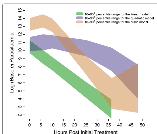
Figure 3 Summaries of simulated log parasite-time profiles used for the evaluation procedure. The green, purple and brown shaded regions represent the 10–90 th percentile ranges of the simulated linear, quadratic and cubic log parasite-time profiles, respectively.
