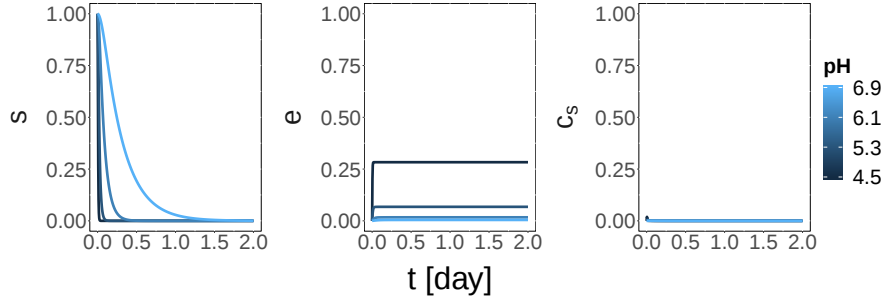
Figure 7.5: Results for the system (Equations (7.14) to (7.19)) at varying pH.
