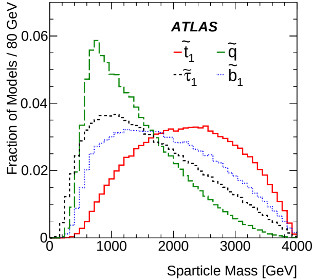
Figure 2: Normalised distribution of sparticle masses for the lightest top (solid red), bottom (dashed blue), first- or second-generation squark (dashed green) and tau (dot-dashed black) for all LSP types combined. The constraints listed in Table 3 have been applied, but not the constraints from the ATLAS searches.
