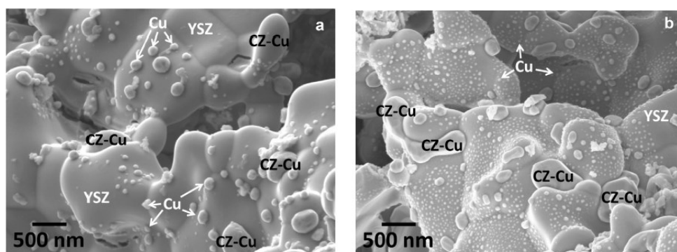
Figure Error! Main Document Only. SEM images of a porous YSZ infiltrated with 10wt% Cu and 20 wt% CZ, before a) and after oxidation at 700 °C and subsequent reduction b). Reprinted with permission from Journal of Power Sources 2014 , 270, 79. Copyright 2014 Elsevier.
