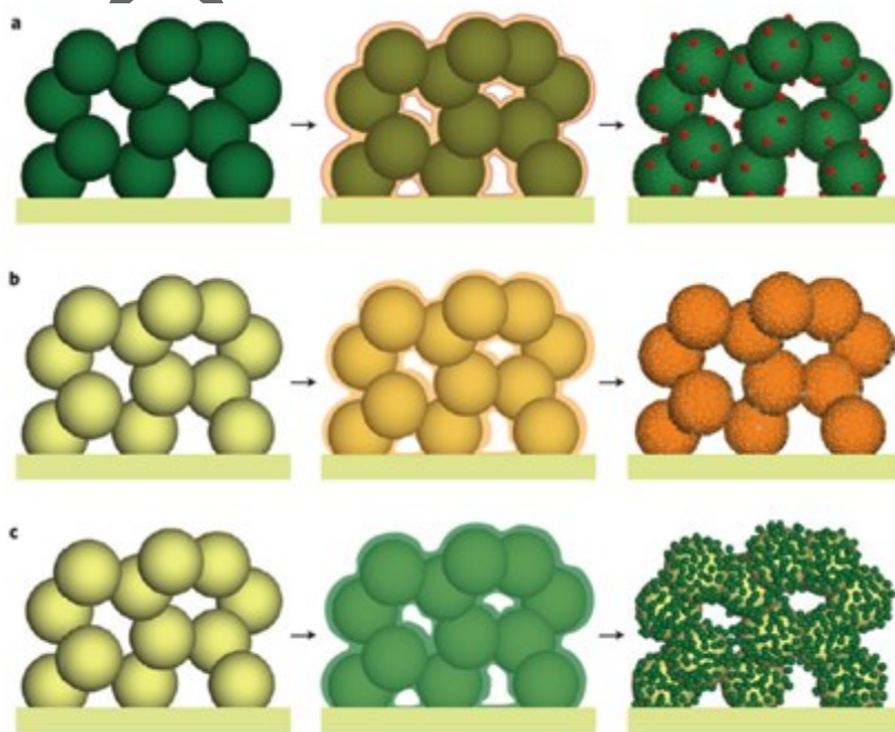
Figure Error! Main Document Only. Examples of microstructures evolved from impregnation a) An electron conducting backbone (green) is infiltrated with precursor (orange) which forms dispersed catalyst particles across the surface. This can be a single material or multiple phases. b) An ionic conducting backbone (yellow) is coated with precursors, which will form a continuous electron or mixed ion electron conducting perovskite phase (orange). In some cases surface morphology may change with atmosphere to increase triple phase boundary. c) An ionic conducting backbone (yellow) is coated with precursors, which will form a percolating network of electronic conducting particles. [Modified from Ref.13]
