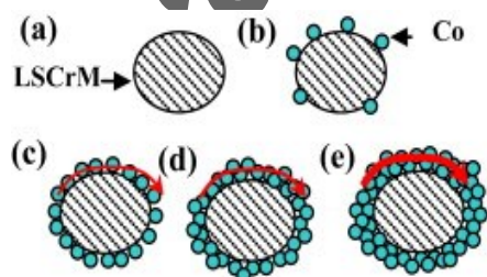
Figure Error! Main Document Only. Model of LSCM backbone impregnated with: (a) 0 mg cm -2 Co, (b) 0.56 mg cm -2 Co, (c) 1.66 mg cm -2 Co, (d) 2.22 mg cm -2 Co, (e) 3.88 mg cm -2 Co. Reprinted with permission from International Journal of Hydrogen Energy 2014 , 39, 7980. Copyright 2014 Elsevier.
