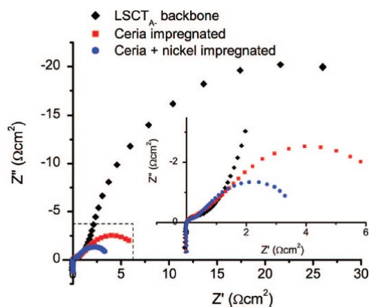
Figure Error! Main Document Only . Cell impedance from LSCT A - backbone with either 10 wt% CeO 2 or with 10 wt% CeO 2 + 5 wt% Ni at 900 °C in H 2 with 1% H 2 O at OCV. Reprinted with permission from J. Electrochem. Soc. 2012, 159, F757. Copyright 2012 The Electrochemical Society.
