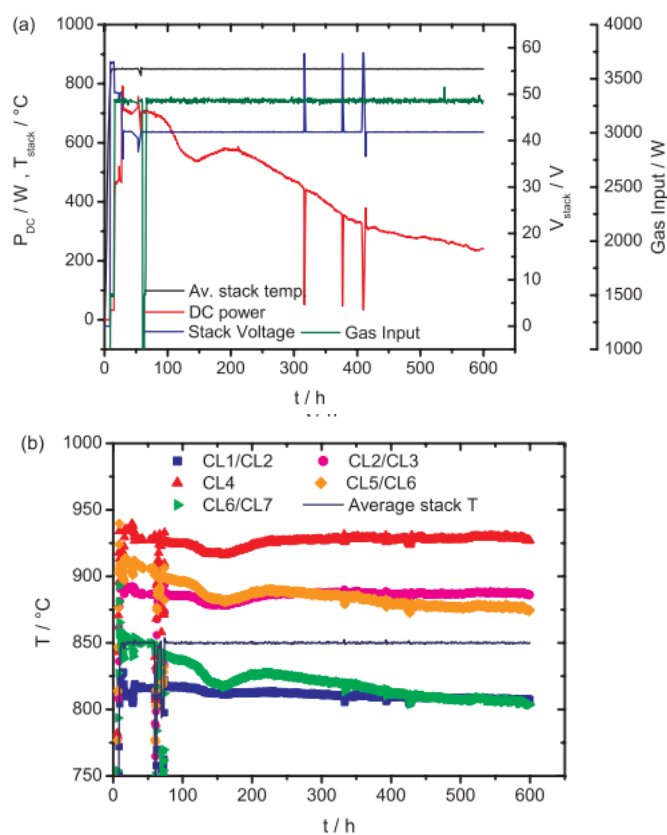
Figure Error! Main Document Only.. Results from Hexis Galileo system test with LSCT A anodes impregnated with Ni + GDC a), and monitored Cluster temperatures during test b) which shows large thermal gradient across stack, with central clusters (CL3, CL4, CL5) displaying temperatures up to 100 ^\circ C higher than external clusters (CL1 and CL7). Reproduced with permission from Fuel Cells 2015, 15, 682. Copyright 2015 Wiley.
