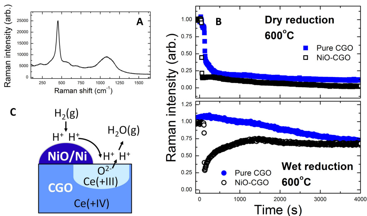
Figure Error! Main Document Only. A: An example Raman spectrum of CGO-NiO cermet in-situ at 600°C. B: Example in-situ Raman monitoring of the reduction of CGO-NiO cermet and pure CGO in dry and wet (humidified to 3% \text{H}_2\text{O} ) hydrogen. CGO reduces faster and to a greater extent when combined with NiO. This is due to the spillover of hydrogen from the Ni to the CGO at the TPB and the effect of the hydrogen spillover over the TPB is even larger in the wet gas.. C: Schematic illustration of the hydrogen spillover process. . Adapted from Advanced Science, 2016 3 (1), 1500146 (CC BY 4.0)
