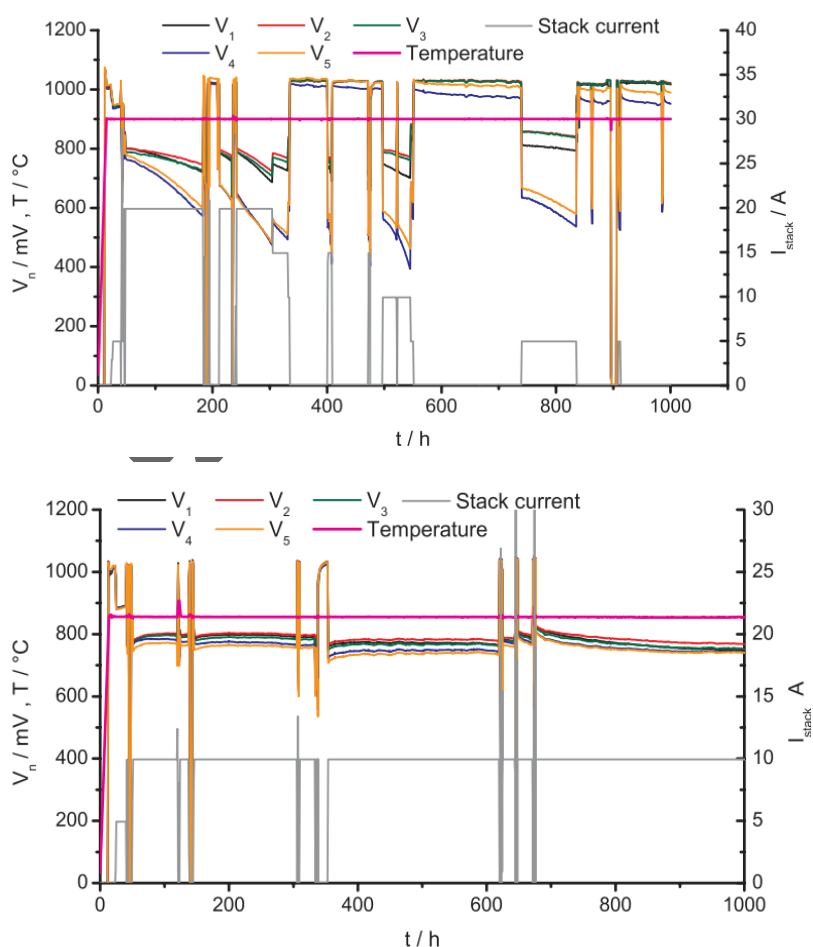
Figure Error! Main Document Only. Stability tests of 5 cell stack with LSCT A anode with Ni+CeO 2 as impregnated catalysts at 900 °C in 4 g h -1 of CPOx (catalytic partial oxidation) reformed natural gas a) and that with Ni + GDC as impregnated catalysts at 850 °C b) in the identical gas conditions. Reproduced with permission from Fuel Cells 2015, 15 , 682. Copyright 2015 Wiley.
