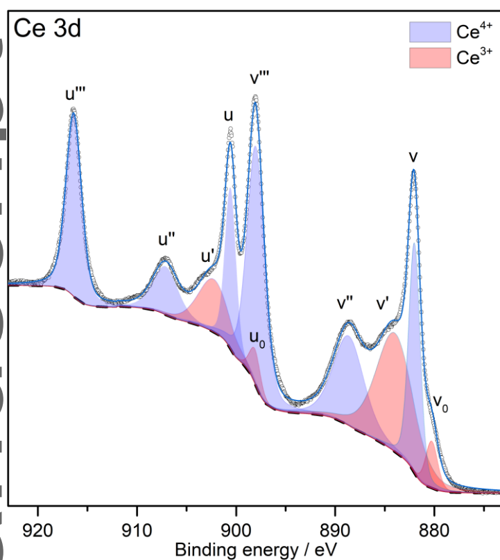
Figure Error! Main Document Only.. Ce 3d XPS spectra from the \text{CeO}_2 infiltrated on porous YSZ (dots), fit (solid blue line), Shirley-type background (dashed line), and components assign to \text{Ce}^{4+} (light blue) and \text{Ce}^{3+} (light red).
