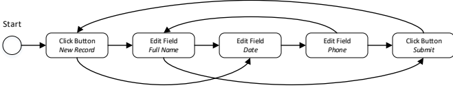
Fig. 2: Example of a Control-Flow Graph
