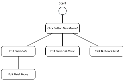
Fig. 3: Dominator tree
