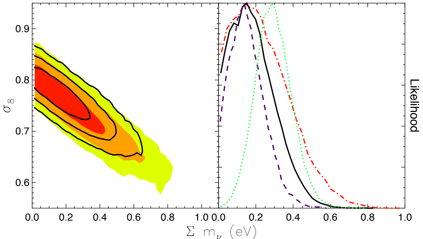
FIG. 8.— Left panel: 2D likelihoods for \sigma_8 and \sum m_\nu . The filled colored contours show the 1, 2, and 3 \sigma constraints for the CMB + H0 + BAO data. The black solid lines show the constraints with the addition of the tSZ information (assuming a 50% theory prior). Right panel: 1D likelihoods for the sum of neutrino masses for four cases. The red dot-dash line shows the constraints without including tSZ data. The black solid line shows the constraints when we include the measured tSZ power with the Shaw tSZ model and a 50% theory prior. This tightens the upper limit on the sum of the neutrino masses from 0.52 eV to 0.40 eV at 95% CL. We show the constraints on neutrino mass that would be derived with perfect tSZ modeling in the final two lines: with the Shaw tSZ model (purple dashed line) and Sehgal tSZ model (green dotted line). The Sehgal model predicts more tSZ power for a given \sigma_8 . As a result it pushes the allowed parameter volume to lower \sigma_8 and higher \sum m_\nu , leading to a nominal detection of the total neutrino mass at 0.29 \pm 0.10 eV.
