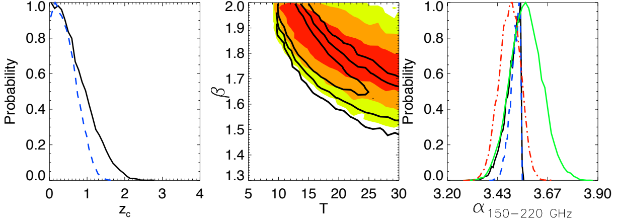
FIG. 12.— CIB frequency modeling. Left panel: Constraint on the mean source redshift with the simple Single SED model parametrized with T = 35 \text{ K} , \beta = 2 , and \sigma_z = 2 . The redshift constraints with and without the HFI 353 GHz data included are plotted in blue dashed and black lines respectively. Middle panel: 2D likelihood surface for T and \beta for the modified black-body CIB spectrum with 95-220 GHz data ( shaded contours ) and 95-353 GHz data ( line contours ). Right panel: The effective CIB spectral index for 150 - 220 GHz. For the Single SED model frequency scaling, the preferred spectral indices are plotted in black solid and blue dashed lines for 95-220 GHz and 95-353 GHz respectively. The sharp cutoff near \alpha = 3.55 is the z_c > 0 prior in the Single SED model. The spectral index constraints with the modified black-body model with and without 353 GHz are shown by the red dot-dashed and green solid lines respectively.
