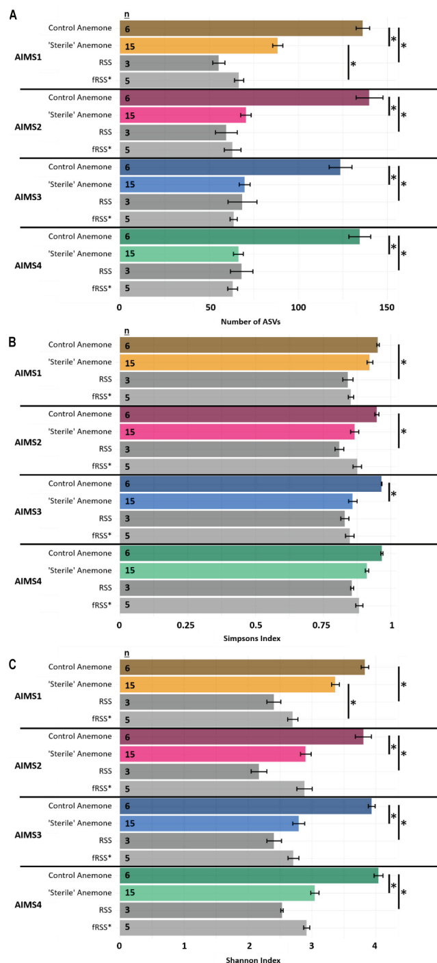
FIGURE 1 | Observed ASVs (A), Simpson's Index (B), and Shannon's Index (C) for AIMS1-4 anemones (orange, purple, blue, green) and seawater (gray) samples in control (unfiltered seawater) or sterilized seawater (SW). The data set was rarefied to 16,993 reads per sample with technical triplicates pooled. Asterisks indicate significant pairwise differences between sample types by genotype. Averages \pm SE are shown. Statistical output for pairwise comparisons is in Supplementary File S3 . *fRSS was collected after hosting anemones for 7 days.
