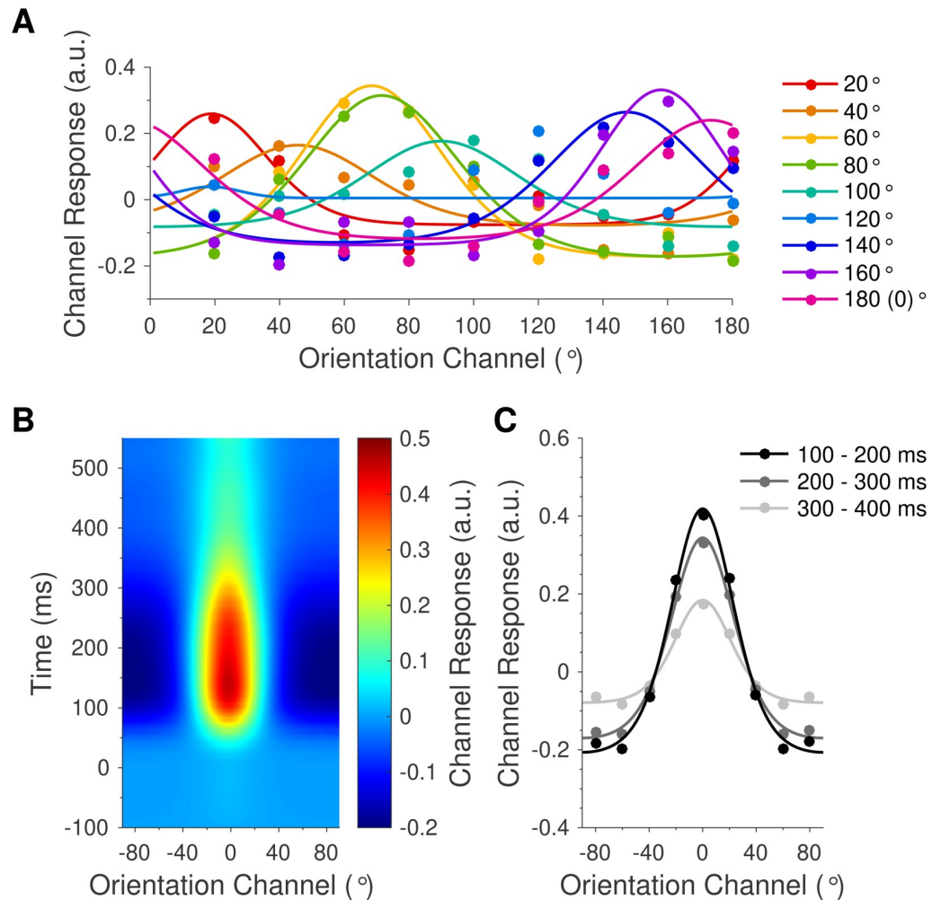
Fig 2. Stimulus-evoked orientation channel response profiles. (A) Reconstructed orientation channels, corresponding to each of the nine grating orientations presented to participants ( 0^{\circ} – 160^{\circ} , in 20^{\circ} steps). Coloured dots indicate the modelled orientation channel activity across trials in which the labelled orientation was presented. Curved lines show functions fitted to the grand average data for illustrative purposes. Note that each coloured line is approximately centred on the presented orientation. (B) Time-resolved orientation response profile, centred on the presented orientation in each trial and averaged across participants and conditions. Orientation response profiles emerged shortly after stimulus onset and lasted until the end of the epoch. (C) Orientation response profiles, averaged across all participants and conditions in each of three successive 100 ms time windows. Dots show activation in each of the nine modelled orientation channels (mean-centred). Curved lines show functions fitted to the grand average data for illustrative purposes. Orientation information (response profile amplitude) was strongest from 100–200 ms and decreased throughout the epoch. Data are available at https://doi.org/10.17605/osf.io/a3pfq . a.u., arbitrary units.
