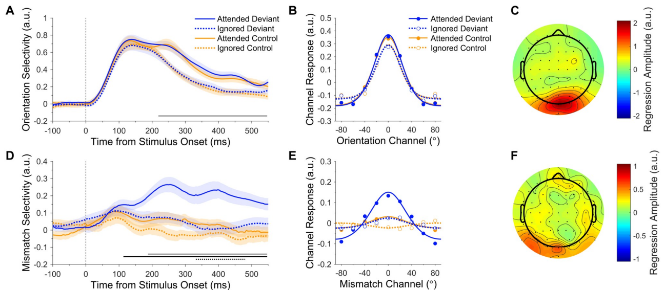
Fig 3. Effects of attention and prediction error on orientation and mismatch response profiles. (A–C) Orientation response profiles. (A) Orientation selectivity (response profile amplitude) for each condition over time. Shading indicates the SEM. The grey bar along the x-axis indicates the main effect of attention (cluster-corrected). (B) Orientation response profiles, averaged across the significant effect of attention shown in A (219–550 ms). Dots show activation in each of the nine modelled mismatch channels. Curved lines show functions fitted to channel responses (fitted to grand average data for illustrative purposes). (C) Univariate sensitivity for stimulus orientation across all conditions (see Methods ). Topography shows the permutation-corrected z-scores, averaged across the significant effect of attention shown in A (219–550 ms). Posterior electrodes were the most sensitive to orientation information. (D–F) mismatch response profiles (observed minus predicted orientation). (D) Mismatch selectivity (response profile amplitude) for each condition over time. Bars along the x-axis indicate the main effect of attention (grey bar, top), the main effect of prediction (black bar, middle), and the interaction (dotted black bar, bottom). Attention enhanced the mismatch response profile in response to deviants but not controls. (E) mismatch response profiles, collapsed across the significant interaction shown in D (332–480 ms). (F) Univariate sensitivity for mismatch response profiles evoked by attended deviants (see Methods ), averaged across 332–480 ms. Posterior electrodes were the most sensitive to mismatch information. Note that C and F use different scales. Data are available at https://doi.org/10.17605/osf.io/a3pfq . a.u., arbitrary units.
