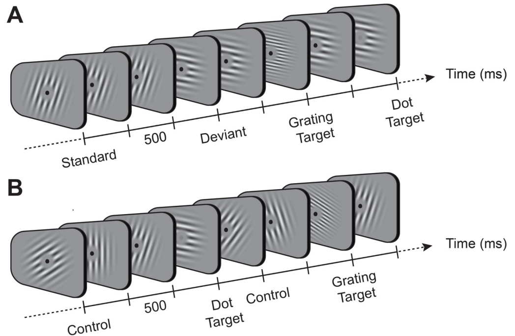
Fig 1. Example stimuli in each of the two block types used in the study. (A) Roving oddball sequence. In this sequence, the orientation of gratings was repeated over short sequences of stimuli ('standards'), before changing to a different orientation ('deviant'). During the grating or dot task, participants responded to rare gratings with high spatial frequency ('grating target') or to rare decreases in fixation-dot contrast ('dot target'), respectively. (B) Equiprobable sequence. In this sequence, the orientation of control gratings changed with each successive presentation.
