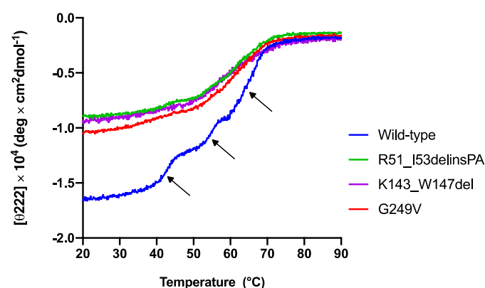
Figure 3. Thermal unfolding profiles of wild-type and mutant MBP-CHIP proteins monitored by circular dichroism spectroscopy. Thermal unfolding curves were obtained for MBP-CHIP proteins by following changes in molar ellipticity at 222 nm wavelength as a function of temperature. Wild-type MBP-CHIP shows three distinct transitions at approximately 42.8 °C, 54.6 °C, and 65.1 °C, as indicated by arrows, whereas all three variants show loss in both ellipticity and transitions.
