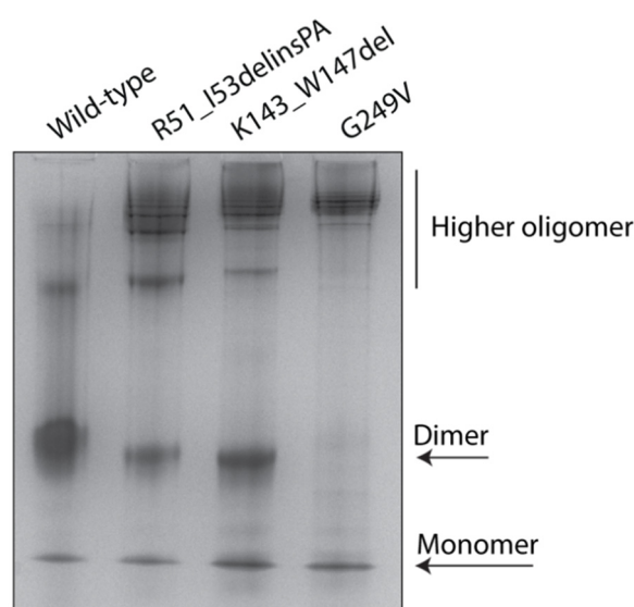
Figure 4. Oligomerization states of wild-type and mutant MBP–CHIP proteins. Native structures of 5 µg MBP–CHIP proteins were studied by native–PAGE on a 10% gel. Protein bands were visualized by Coomassie blue staining and analyzed by Fiji (ImageJ) software [15].
