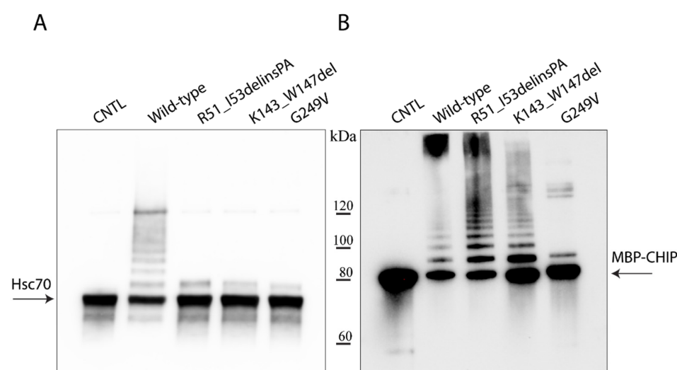
Figure 2. Ubiquitination activity of wild-type and mutant MBP-CHIP proteins. In vitro ubiquitination activity test was performed on MBP-CHIP recombinant proteins using Hsc70 (A) and MBP-CHIP (B) as the substrates. A separate wild-type reaction without ubiquitin was used as the negative control (CNTL) for each assay.
