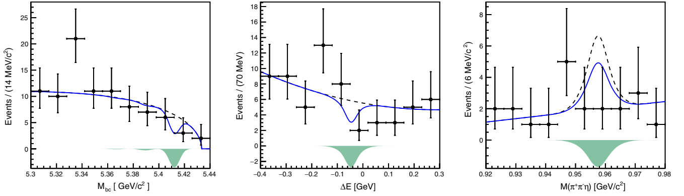
FIG. 2. Signal region fit projections onto M_{bc} , \Delta E and M(\pi^+\pi^-\eta) for B_s^0 \rightarrow \eta'K_S^0 event candidates in \Upsilon(5S) data after additional selection criteria are applied, as described in the text. Points with the error bars show the binned data. Blue solid lines show the results of the fit, filled area and black dashed line show the signal and background fit components, respectively.
