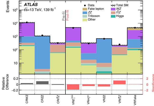
FIG. 5. The observed data and the SM background expectation in the CRs (prefit) and VRs (postfit). The “other” category consists mostly of the tWZ , t\bar{t}W , and tZ processes. The hatched bands indicate the combined theoretical, experimental, and MC statistical uncertainties in the background prediction. The bottom panel shows the fractional difference between the observed data and expected yields for the CRs and the significance of the difference for the VRs, computed following the profile likelihood method described in Ref. [102].
