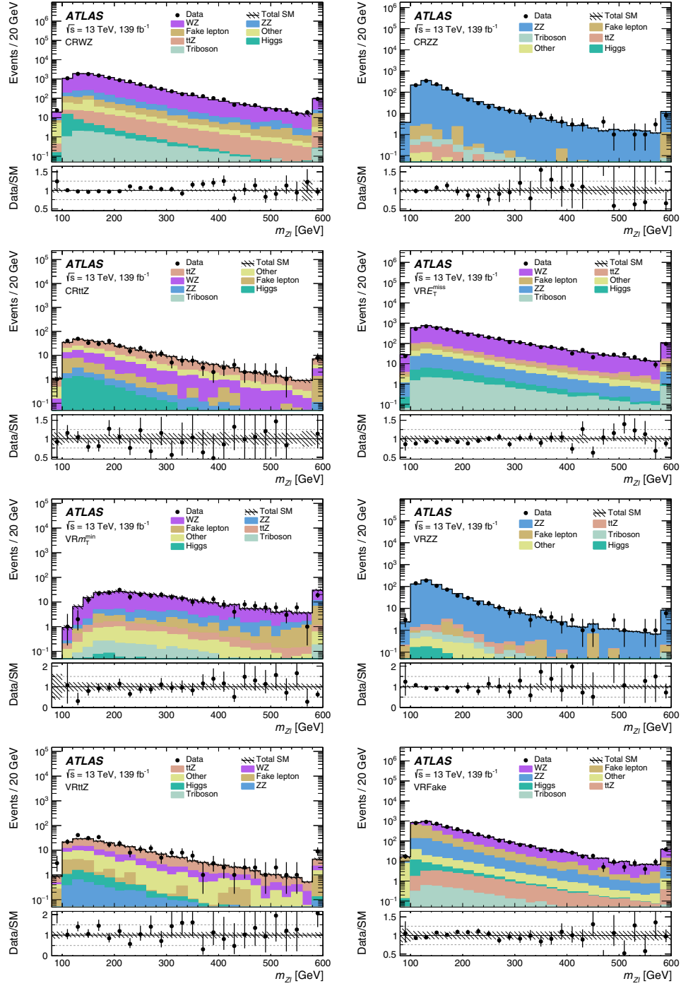
FIG. 4. The m_{Z\ell} distributions of the data and postfit background in the (from top left to bottom right) CRWZ, CRZZ, CR \bar{t}Z , VRE_T^{\text{miss}} , VRm_T^{\text{min}} , VRZZ, VR \bar{t}Z , and VRFake regions. The last bin includes overflow events. The “other” category consists mostly of the tWZ , \bar{t}\bar{t}W , and tZ processes. The hatched bands indicate the combined theoretical, experimental, and MC statistical uncertainties in the background prediction. The bottom panel shows the ratio of the data to the background prediction.
