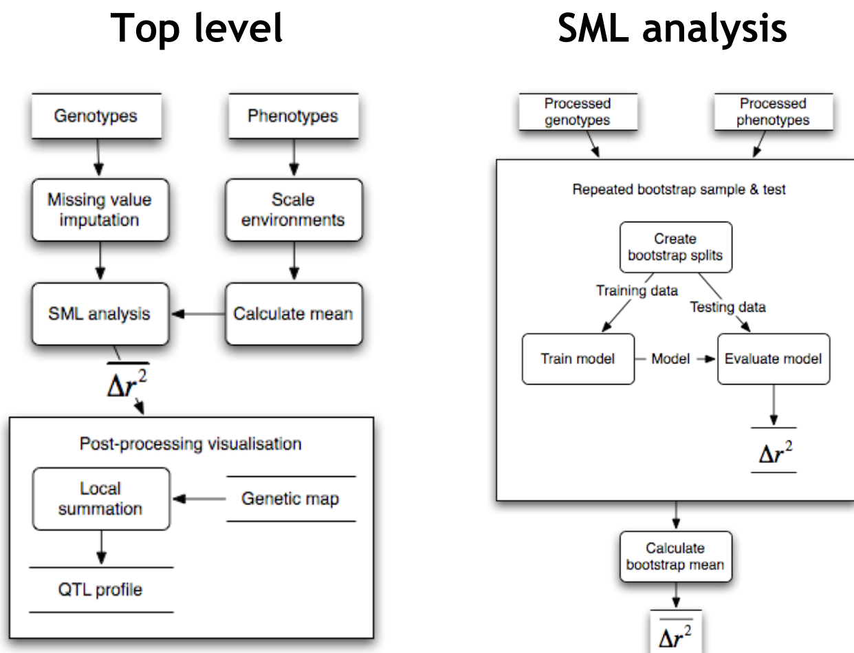
Figure 1 System dataflow diagram. Dataflow diagram (DFD) depicting the QTL analysis. Rectangles with round corners indicate processes, other rectangles indicate data stores, and lines indicate data flow. The left figure shows the top-level DFD, the right shows further detail of the 'SML analysis' process.
