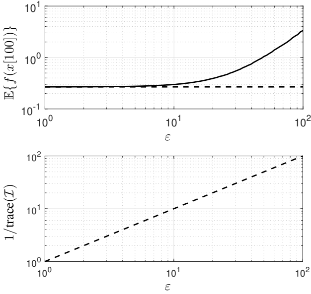
Fig. 1. [top] \mathbb{E}\{f(x[100])\} versus \varepsilon after 100 iterations of (3) (solid) and \min_{x \in \mathcal{C}} f(x) (dashed). [bottom] 1/\text{trace}(\mathcal{I}) versus \varepsilon .
