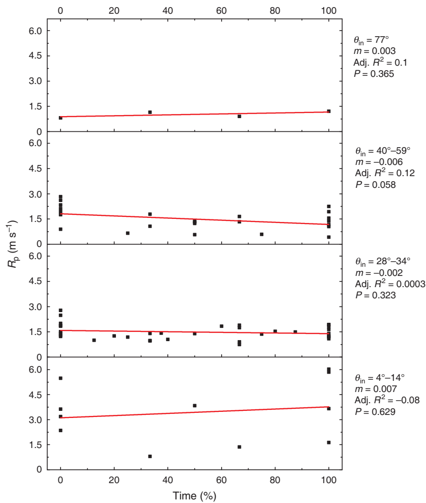
Fig. 9. Variation of the rate of spread R_p of the intersect point of two junction fire fronts. Angles in the legend indicate the value at the initial time, m is the slope of the regression line, Adj. R^2 is the adjusted R^2 , P is the significance value. R_p at the 100% time step corresponds to the last time the angle between junction fire fronts became 180^\circ .
