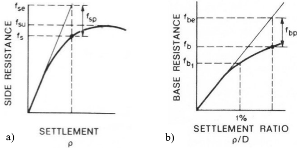
Figure 2. Principles for normalising (a) side resistance and (b) base resistance (after Williams et al, 1980, with permission from Taylor and Francis).
