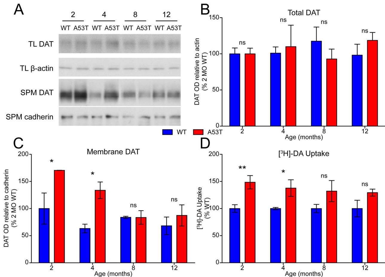
Figure 3. DAT distribution and function. Expression and distribution of DAT was analyzed by immunoblot on protein from (A) total lysates (TL) or synaptosomal plasma membrane fractions (SPM). Actin or cadherin expression, respectively, were analyzed as loading controls. Representative blot images from each genotype at each age are presented with approximate molecular mass of nearest protein ladder bands indicated (M r ). Band optical density (OD) of (B) TL and (C) SPM DAT relative to loading controls is presented as percent of two month-old WT (mean \pm SEM) and was analyzed by two-way ANOVA with Bonferroni post-hoc tests comparing each A53T group to age-matched controls (* p <0.05). (D) Uptake of [ 3 H]-DA into striatal synaptosomes isolated from WT and A53T mice at 2–12 months of age was measured in triplicate from six animals per group and is presented as percent of age-matched WT control (mean \pm SEM). Non-specific uptake was determined in the presence of 100 \mu M indatraline HCl and has been subtracted. Comparisons between WT and A53T \alpha -Syn at each age were made by t-test (* p <0.05, ** p <0.01). doi:10.1371/journal.pone.0060378.g003
