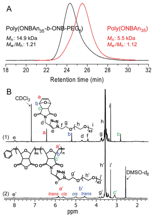
Fig. 1 Characterization of linear-brush diblock copolymers poly(OBAN 35 - b -ONB-PEG 5 ) (A) GPC measurements and (B) 1 H NMR spectroscopic analysis.
