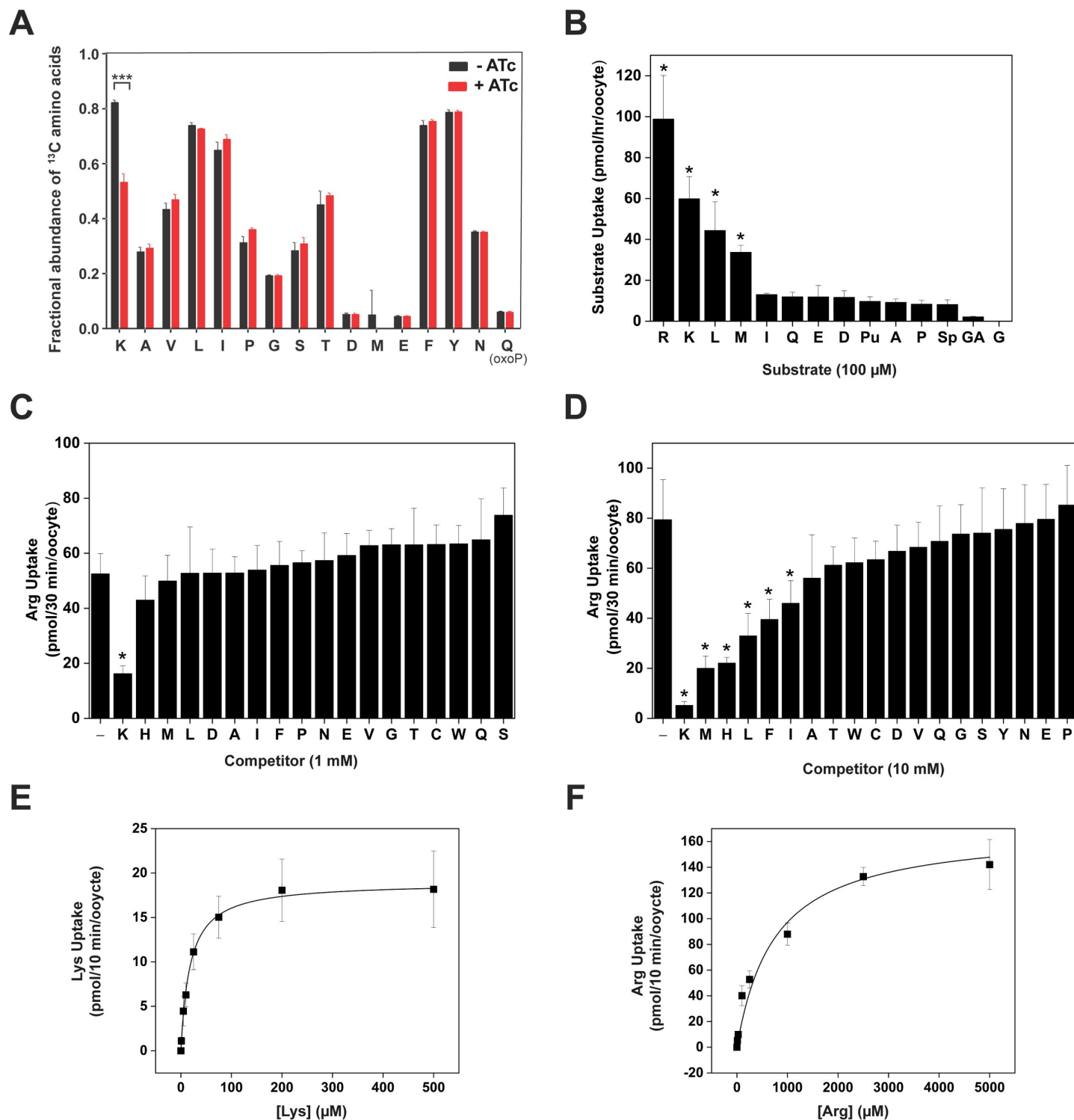
Fig 2. TgApiAT6-1 is a cationic and neutral amino acid transporter with high affinity for Lysine. A. Analysis of [ ^{13}\text{C} ] amino acid uptake in parasites expressing or lacking TgApiAT6-1. rTgApiAT6-1 parasites were cultured for 2 days in the absence (black) or presence (red) of ATc until natural egress, then incubated in medium containing [ ^{13}\text{C} ]-L-amino acids for 15 min. Metabolites were extracted and the fractions of [ ^{13}\text{C} ]-L-amino acids determined by GC-MS. Amino acids are represented by single letter codes; OxoP, 5-oxoproline. The data represent the mean \pm S.D. of 3 replicate experiments (*, P < 0.001 , Student's t test. Where significance values are not shown, differences were not significant; P > 0.05 ). B. Uptake of a range of amino acids into oocytes expressing TgApiAT6-1. Uptake was measured in the presence of 100 \mu\text{M} unlabelled substrate and 1.0 \mu\text{Ci/ml} [ ^3\text{H} ] or [ ^{14}\text{C} ] substrate. Amino acid substrates are represented by single letter codes, while for other metabolites: Pu, putrescine; Sp, spermidine; and GA, \gamma -amino butyric acid (GABA). Each bar represents the mean \pm S.D. uptake of 10 oocytes for a single experiment, and each is representative of three independent experiments. The uptake
