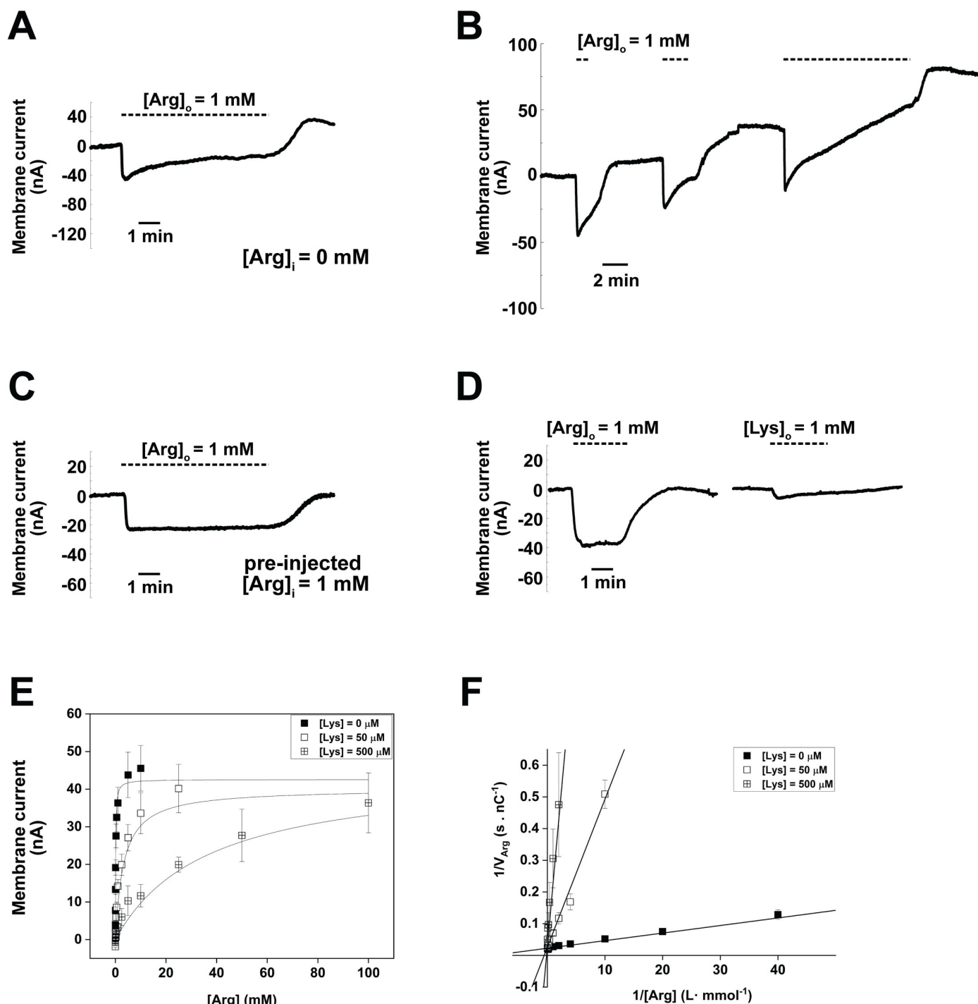
Fig 3. Arg and Lys compete for the same binding site in TgApiAT6-1. Electrophysiology measurements in TgApiAT6-1 expressing oocytes. All currents were recorded in two-voltage clamp configuration to record membrane current. All oocytes were voltage clamped at -50 mV and the application of substrate (Arg or Lys) are indicated by the dashed horizontal lines above the tracings. Representative current tracings were normalised to 0 nA to remove background (non-substrate induced) current. A. Representative current tracing of TgApiAT6-1 expressing oocytes upon the addition and subsequent washout of 1 mM extracellular Arg ([Arg] o ) with no pre-injection of substrate. The perfusion buffer used was ND96 (pH 7.3). B. Representative current tracing of a TgApiAT6-1 expressing oocyte repeatedly pulsed with 1 mM Arg for 1 min, 2 min, and 10 min with 5 min gaps in between pulses. The perfusion buffer used was ND96 (pH 7.3). C. Representative current tracing of a TgApiAT6-1 expressing oocyte pre-injected with 1 mM Arg ([Arg] i = 1 mM) upon the addition and subsequent washout of 1 mM extracellular Arg ([Arg] o ). The perfusion buffer used was ND96 (pH 7.3). D. Representative current tracings of TgApiAT6-1 expressing oocytes upon the addition and subsequent washout of either 1 mM extracellular Arg ([Arg] o ) or Lys ([Lys] o ) with no pre-injection of substrate. The perfusion buffer used was ND96 (pH 7.3). E-F. Inhibition kinetics of increasing [Lys] on Arg-induced inward currents in TgApiAT6-1 expressing oocytes. All oocytes were voltage-clamped at -50 mV and
