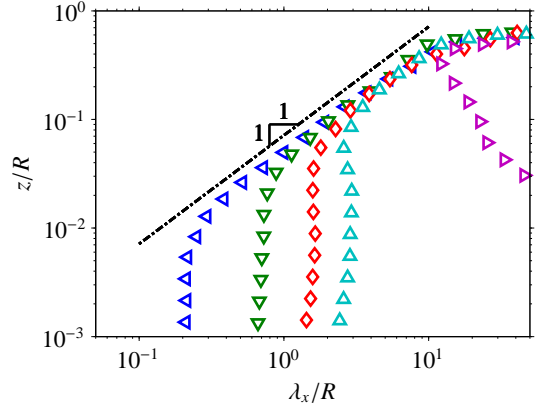
Figure 13: \gamma_L^2 = 0.1 contours between u and u_\tau signals at Re_\tau \approx 40\,000 as function of \Delta s ; \Delta s/R \approx 0 ( \blacktriangleleft ), 0.02 ( \nabla ), 0.03 ( \diamond ), 0.06 ( \triangle ) and 0.13 ( \blacktriangleright ).
