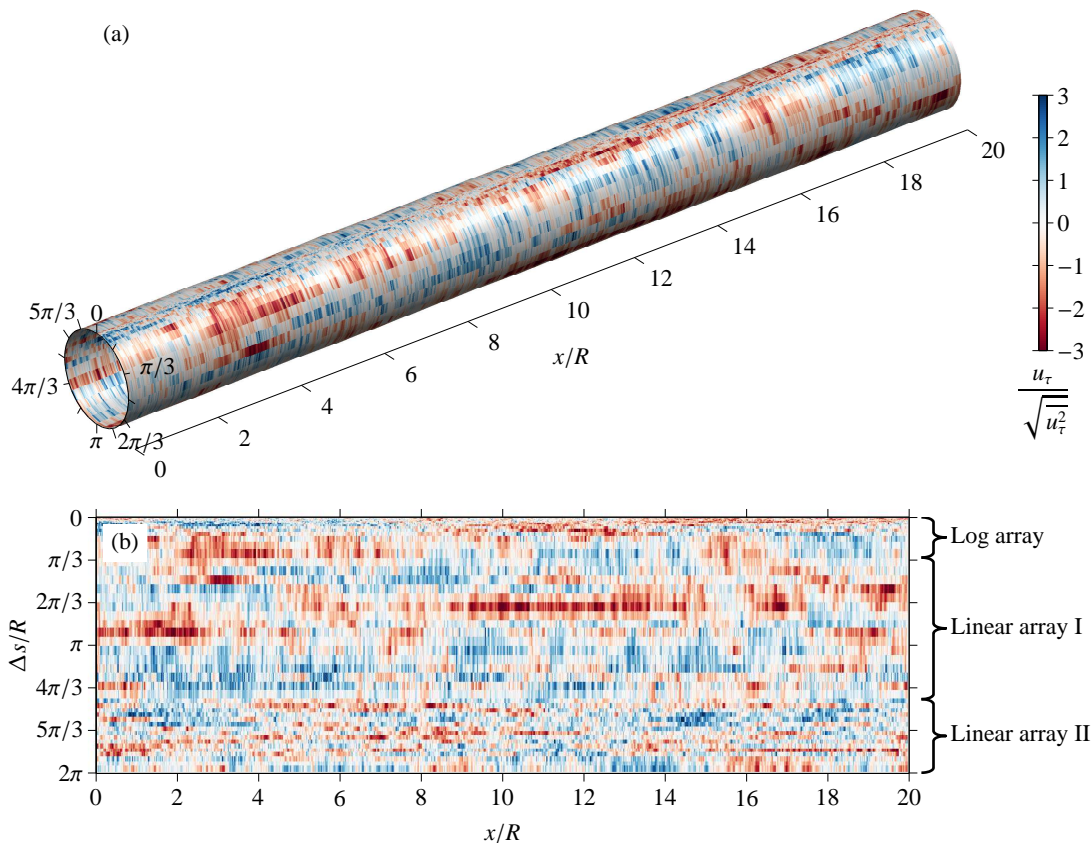
Figure 6: Instantaneous fluctuating friction velocity, u_\tau , recorded by hot-film sensors at Re_\tau \approx 40\,000 . (a) Shows a three-dimensional view of u_\tau along a pipe surface, while its projection on to a flat plane is shown in (b).
