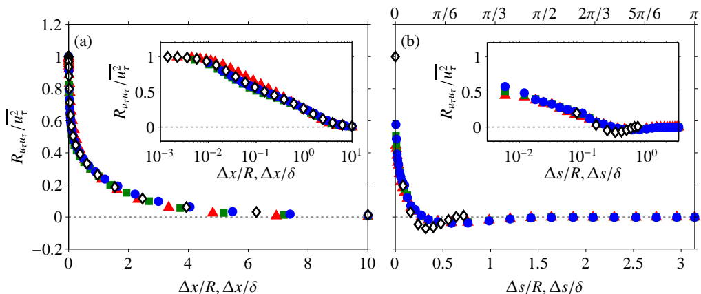
Figure 5: Two-point correlation of fluctuating friction velocity, R_{u_\tau, u_\tau} . The correlation coefficients are shown as functions of (a) the longitudinal ( R_{u_\tau, u_\tau}(\Delta x, 0) ) and (b) transverse ( R_{u_\tau, u_\tau}(0, \Delta s) ) offsets. The solid symbols correspond to pipe flow at Re_\tau \approx 10\,000 ( \blacktriangle ), 22\,000 ( \blacksquare ) and 40\,000 ( \bullet ), while the open symbols ( \diamond ) correspond to boundary layer flow at Re_\tau \approx 14\,000 . For the insets, a logarithmic scale is used for the displacements, \Delta x and \Delta s , between the two points.
