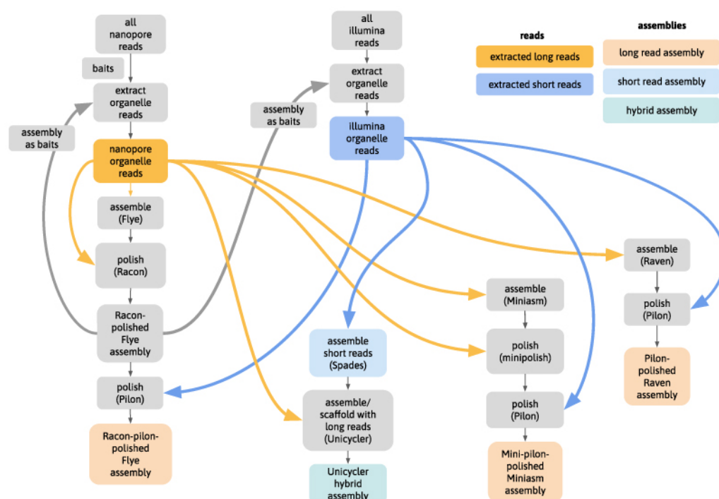
Figure 1. Analysis flowchart. Main steps in the analysis, showing use of initial assembly as baits for further read extraction, and use of read sets in assembly polishing steps.
