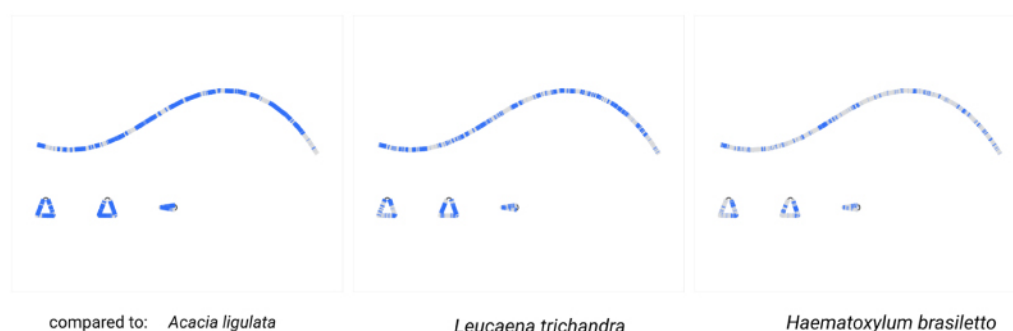
Figure 17. Comparison of the Acacia pycnantha Unicycler assembly with mitomes from related species. The contig is colored according to its match with these assemblies, using the BLAST tool within Bandage. Increasing difference is seen in concert with increasing phylogenetic distance, from left to right.
