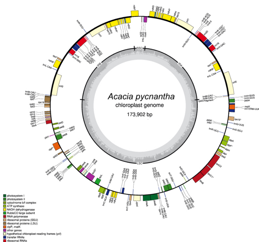
Figure 9. Annotated plastome of Acacia pycnantha , based on Unicycler assembly, and produced by the GeSeq tool and OGDRAW.
