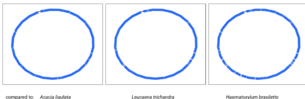
Figure 10. Comparison of the Acacia pycnantha Unicycler assembly with plastomes from related species. The contig is colored according to its match with these assemblies, using the BLAST tool within Bandage. No novel regions or misassembly are evident within A. pycnantha .
