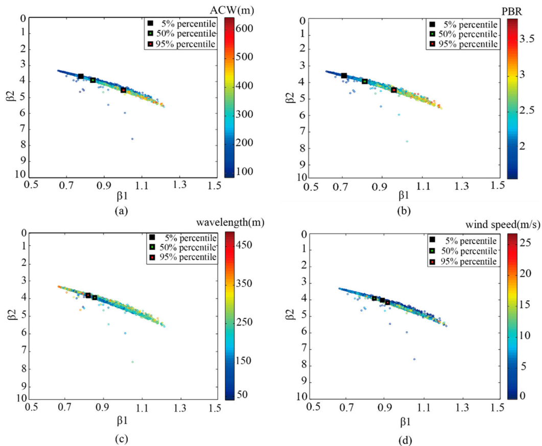
Figure 9. Kurtosis vs. skewness of the samples categorized by (a) ACW, (b) PBR, (c) wavelength, and (d) wind speed.
