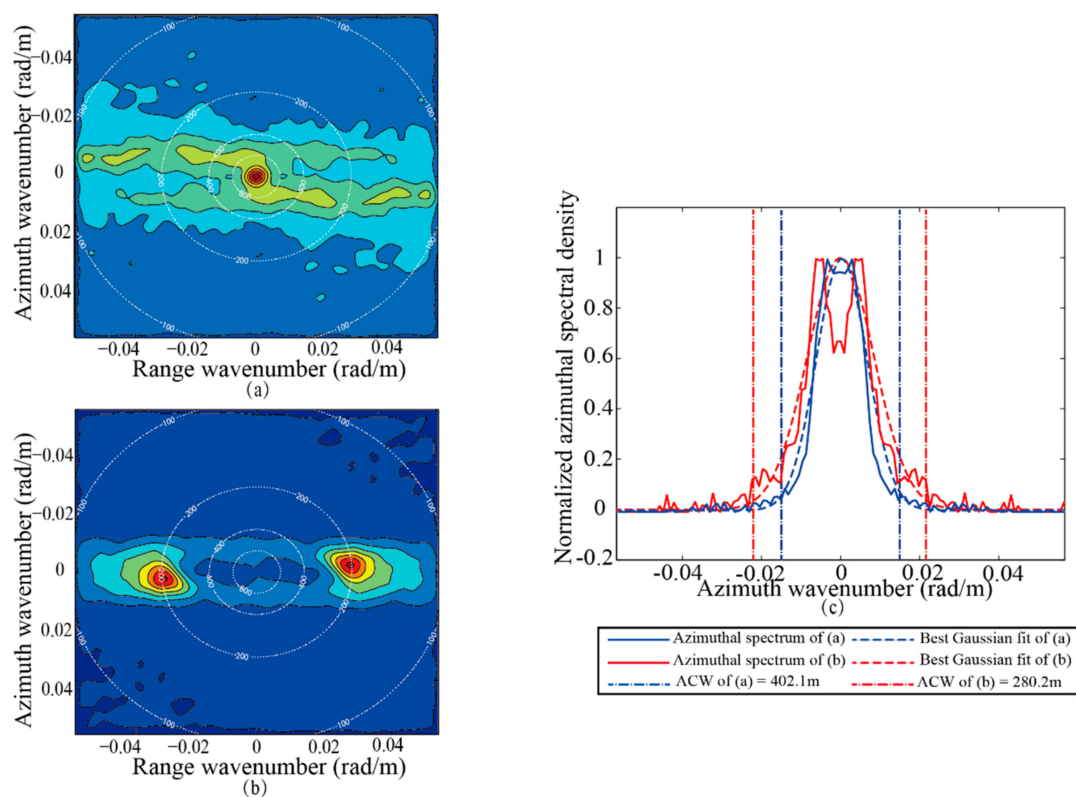
Figure 3. SAR intensity spectra and azimuth cutoff wavelengths (ACWs) for the cases in Figure 2e,f. (a) SAR spectrum corresponding to the image in Figure 2e. The white line is the wavelength isoline. (b) SAR spectrum corresponding to the image in Figure 2f. (c) Estimated ACWs corresponding to (a,b). The solid line is the azimuthal spectrum and the dashed line is the best fit using the Gaussian function. The vertical lines are the estimated ACWs for the two cases.
