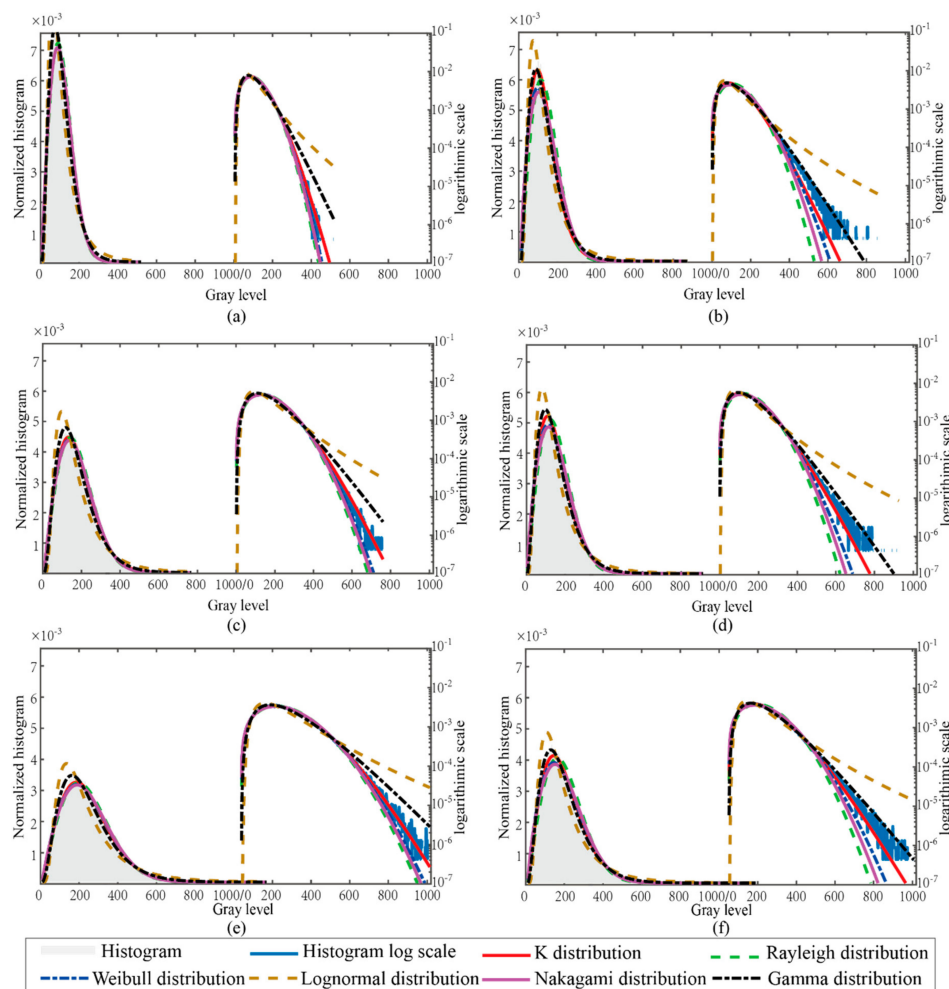
Figure 4. Empirical histogram and fitting results of the SAR images in Figure 2 on linear (left y-axes) and semi-log (right y-axes) scales. (a) Low wind speed (3 m/s) without wave streaks, (b) low wind speed (3 m/s) with wave streaks, (c) moderate wind speed (10 m/s) without wave streaks, (d) moderate wind speed (8 m/s) with wave streaks, (e) high wind speed (17 m/s) without wave streaks, and (f) high wind speed (14 m/s) with wave streaks.
