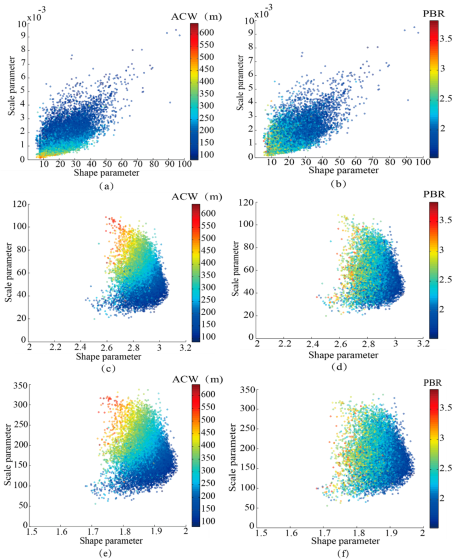
Figure 7. The variations of the distribution parameters with ACW and PBR. (a) K distribution with ACW, (b) K distribution with PBR, (c) Gamma distribution with ACW, (d) Gamma distribution with PBR, (e) Weibull distribution with ACW, and (f) Weibull distribution with PBR. The color shows the ACW or PBR value of the SAR samples.
