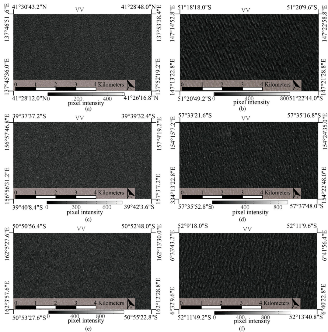
Figure 2. Comparison of the examples of the SAR images indicating the different sea states: (a) Low wind speed (3 m/s) without wave streaks, (b) low wind speed (3 m/s) with wave streaks, (c) moderate wind speed (10 m/s) without wave streaks, (d) moderate wind speed (8 m/s) with wave streaks, (e) high wind speed (17 m/s) without wave streaks, and (f) high wind speed (14 m/s) with wave streaks.
