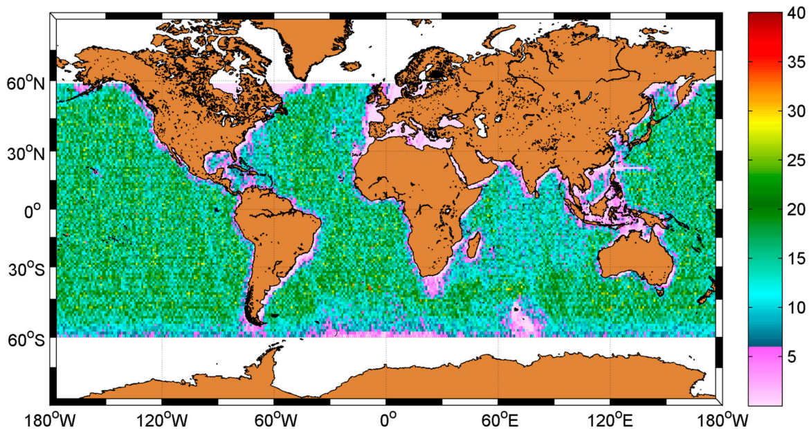
Figure 1. The sample numbers of the Synthetic Aperture Radar (SAR) wave mode imageries for the year, 2010, with a 1^\circ \times 1^\circ spatial grid.
