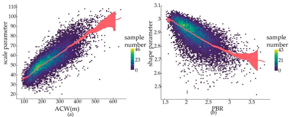
Figure 8. (a) The variations scale parameter with ACW for Gamma distribution; (b) the variations shape parameter with PBR for Gamma distribution. The red line is a smoothed regression of the samples with 95% confidence interval.
