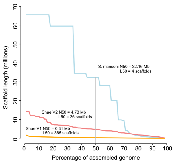
Figure 1: Comparison of schistosome genome assembly quality metrics. Scaffold lengths, N50, and L50 values for Schistosoma haematobium genome version 2 (Shae.V2), version 1 (Shae.V1), and S. mansoni are shown.
