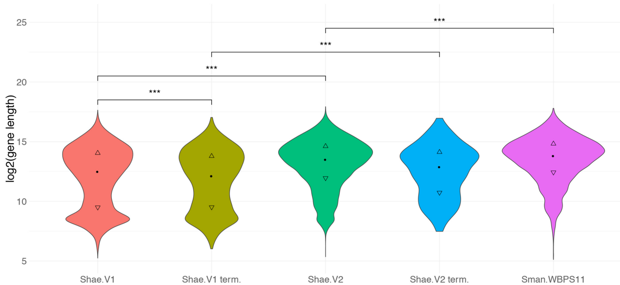
Figure 6: Distribution of gene length for gene sets representing Schistosoma haematobium (Shae.V1 and Shae.V2) and S. mansoni (Sman.WBPS11). Additionally, distributions are shown for terminal genes (i.e., genes encoded at the start or end of a scaffold) for both S. haematobium gene sets (“Shae.V1 term.” and “Shae.V2 term.”). Statistically significant differences among distributions (independent 2-group Mann-Whitney U test) are indicated for P \leq 0.001 (***).
