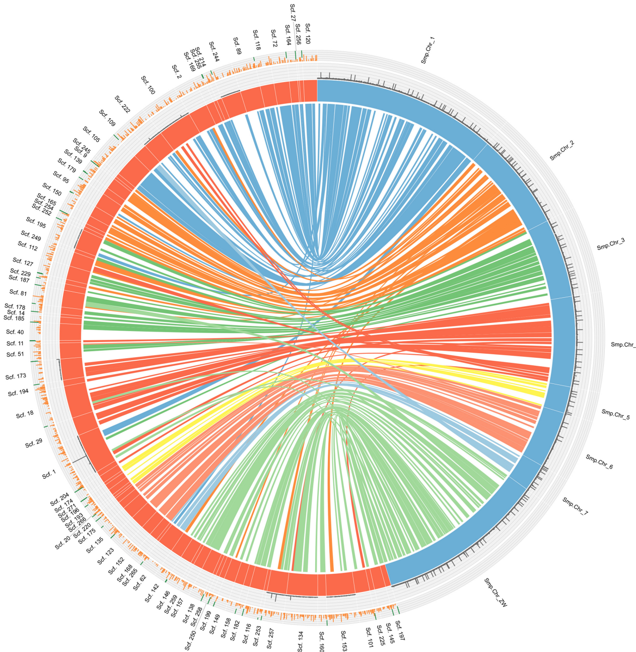
Figure 3: Comparison of the syntenic, contiguity, and integrity of assemblies for S. haematobium version 2 (Shae.V2) and S. mansoni (WBPS8). Shae.V2 scaffolds ( n = 79 ) are represented by orange bars and are linked with 8 S. mansoni chromosomes (light blue bars). Scaffolds are arranged in a circular plot based on 218 regions containing single-copy orthologs (SCOs, each represented by a line connecting an orange with a blue scaffold). SCO lines have distinct colours for each S. mansoni chromosome. Additionally, gaps ("Ns") are represented as black histograms on a separate track, with the Y-axis representing the size of the region containing ambiguous nucleotides (range, 0–5,013). On the outer track, orange histograms represent areas of >1,000 bp in length for which the coverage of "properly paired" reads was <5 reads. Higher histograms represent longer regions. Dark green histograms within the same track represent regions of low "physical" coverage. The lower the histograms "drop" from the top of the track, the larger is the size of the regions that have "physical" coverage of <10 reads.
