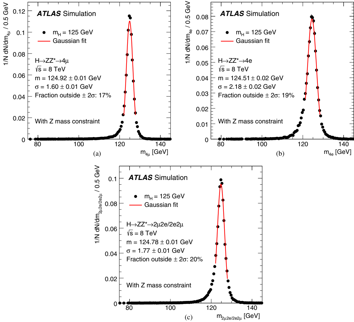
FIG. 12 (color online). Invariant mass distribution for a simulated signal sample with m_H = 125 \, \text{GeV} ; superimposed is the Gaussian fit to the m_{4\ell} peak after the correction for final-state radiation and the Z-mass constraint.
