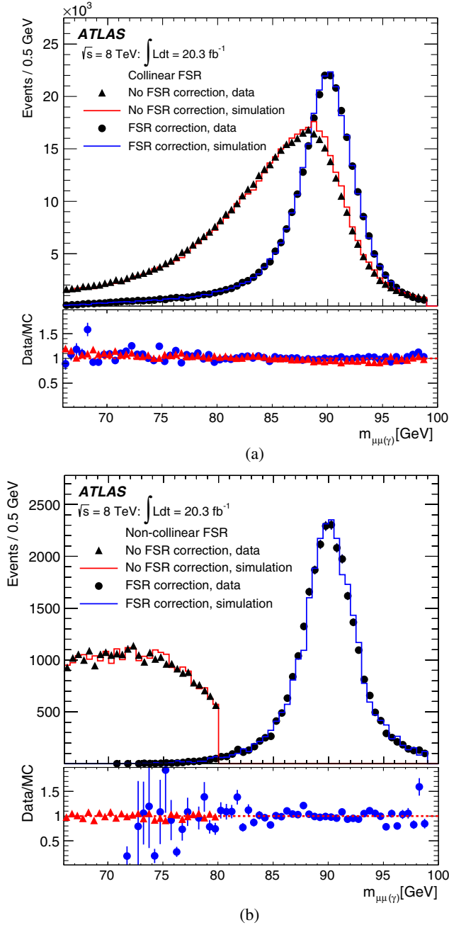
FIG. 1 (color online). (a) The invariant mass distributions of Z \rightarrow \mu^+\mu^-(\gamma) events in data before collinear FSR correction (filled triangles) and after collinear FSR correction (filled circles), for events with a collinear FSR photon satisfying the selection criteria as described in Sec. IV C. The prediction of the simulation is shown before correction (red histogram) and after correction (blue histogram). (b) The invariant mass distributions of Z \rightarrow \mu^+\mu^-(\gamma) events with a noncollinear FSR photon satisfying the selection criteria as described in Sec. IV C. The prediction of the simulation is shown before correction (red histogram) and after correction (blue histogram).
