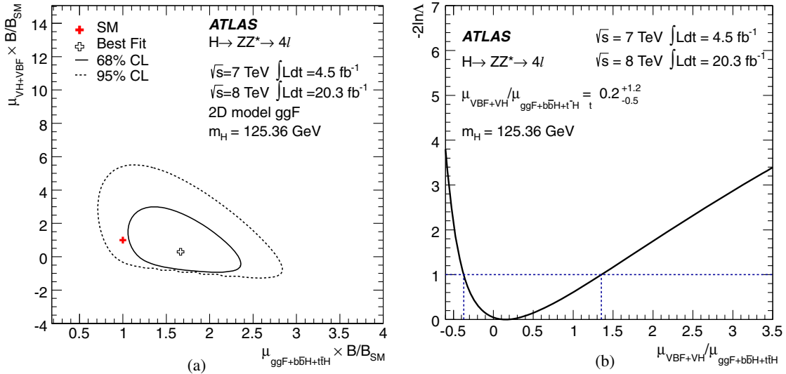
FIG. 20 (color online). (a) Likelihood contours in the (\mu_{\text{ggF+b}\bar{b}\text{H+t}\bar{t}\text{H}}, \mu_{\text{VBF+VH}}) plane including the branching ratio factor B/B_{\text{SM}} . Only the part of the plane where the expected number of signal events in each category is positive is considered. The best fit to the data (open cross) and the 68% CL (solid line) and 95% CL (dashed line) contours are also indicated, as well as the SM expectation (solid red +). (b) Results of a likelihood scan for \mu_{\text{VBF+VH}}/\mu_{\text{ggF+b}\bar{b}\text{H+t}\bar{t}\text{H}} .
