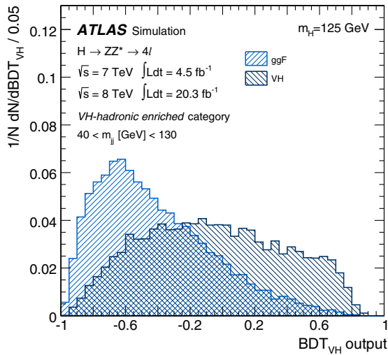
FIG. 10 (color online). Final \text{BDT}_{\text{VH}} discriminant output for the VH-hadronic enriched category for signal (VH events, dark blue) and background (ggF events, light blue) events.
