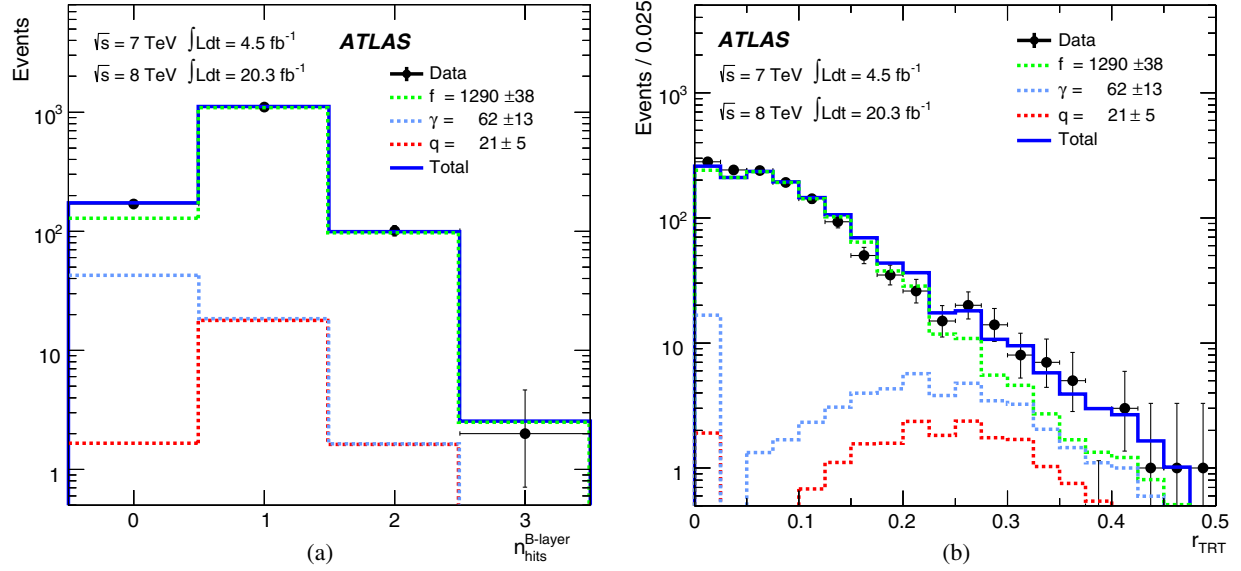
FIG. 6 (color online). The results of a simultaneous fit to (a) n_{\text{hits}}^{\text{B-layer}} , the number of hits in the innermost pixel layer, and (b) r_{\text{TRT}} , the ratio of the number of high-threshold to low-threshold TRT hits, for the background components in the 3\ell + X control region. The fit is performed separately for the 2\mu 2e and 4e channels and summed together in the present plots. The data are represented by the filled circles. The sources of background electrons are denoted as light-flavor jets faking an electron ( f , green dashed histogram), photon conversions ( \gamma , blue dashed histogram) and electrons from heavy-flavor quark semileptonic decays ( q , red dashed histogram). The total background is given by the solid blue histogram.
