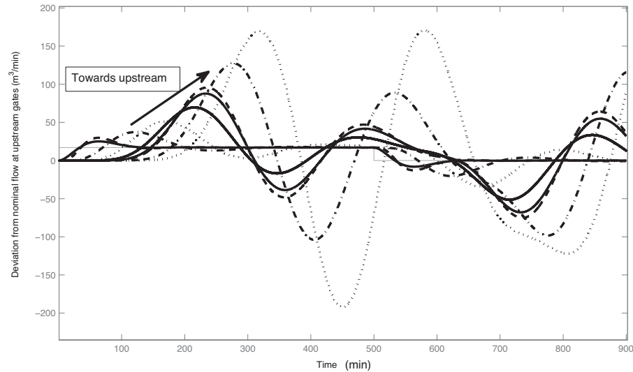
Fig. 3 Response of channel under decentralized distant-downstream control – i.e., F_i(s) = 0 and C_i(s) = K_i \frac{(s+z_i)}{s(s+p_i)} .
