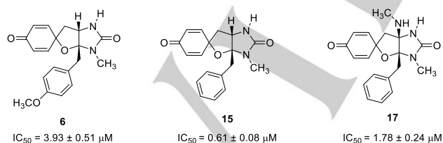
Figure 2. The deletion analogues 5 , 15 and 17 , with the IC_{50} values against the NCI-H522 lung cancer cell line.
