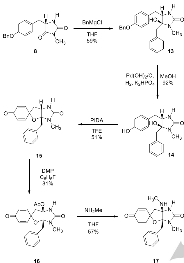
Scheme 3. Synthesis of the C-4 benzyl deletion analogues 15 and 17 .
