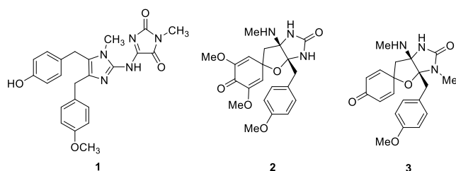
Figure 1. The structures of naamidine A ( 1 ), (+)-spironaamidine ( 2 ) and (-)-spiroleucettadine ( 3 ).
