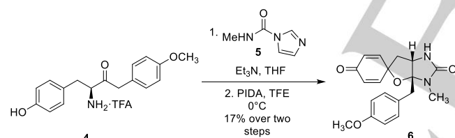
Scheme 1. Original strategy used to access the spirocyclic cyclohexadienone core of spiroleucettadine. [5a]
